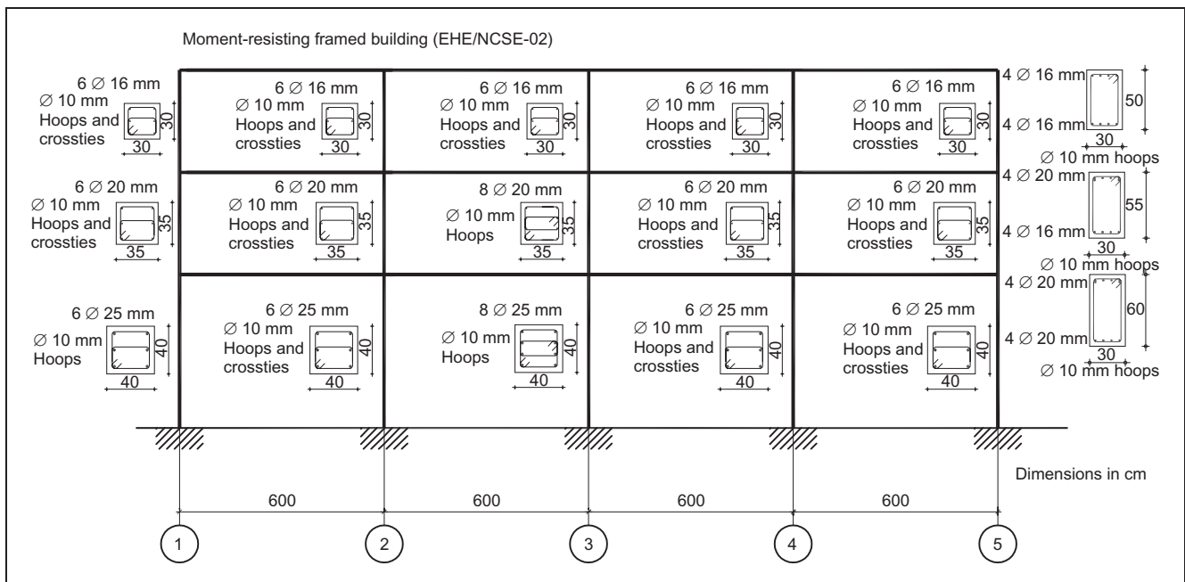
Figure 23. Details of the moment-resisting frame designed according to EHE/NCSE-02 codes
