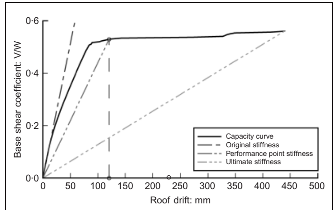
Figure 15. Roof drift corresponding to the performance point of the building with moment-resisting frames (NCSE-02 code)
