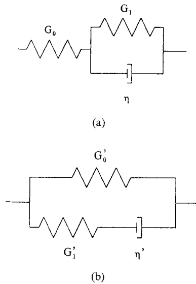
Figure 8.6: Two equivalent schemes of the Zener's solid
