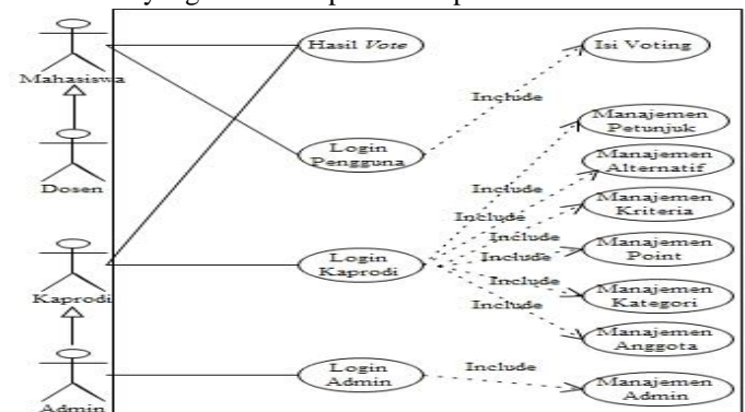
Gambar 3. Usecase Diagram
