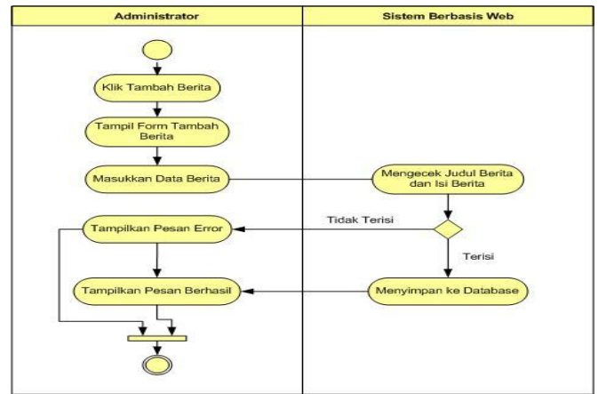
Gambar 2. Activity Diagram
