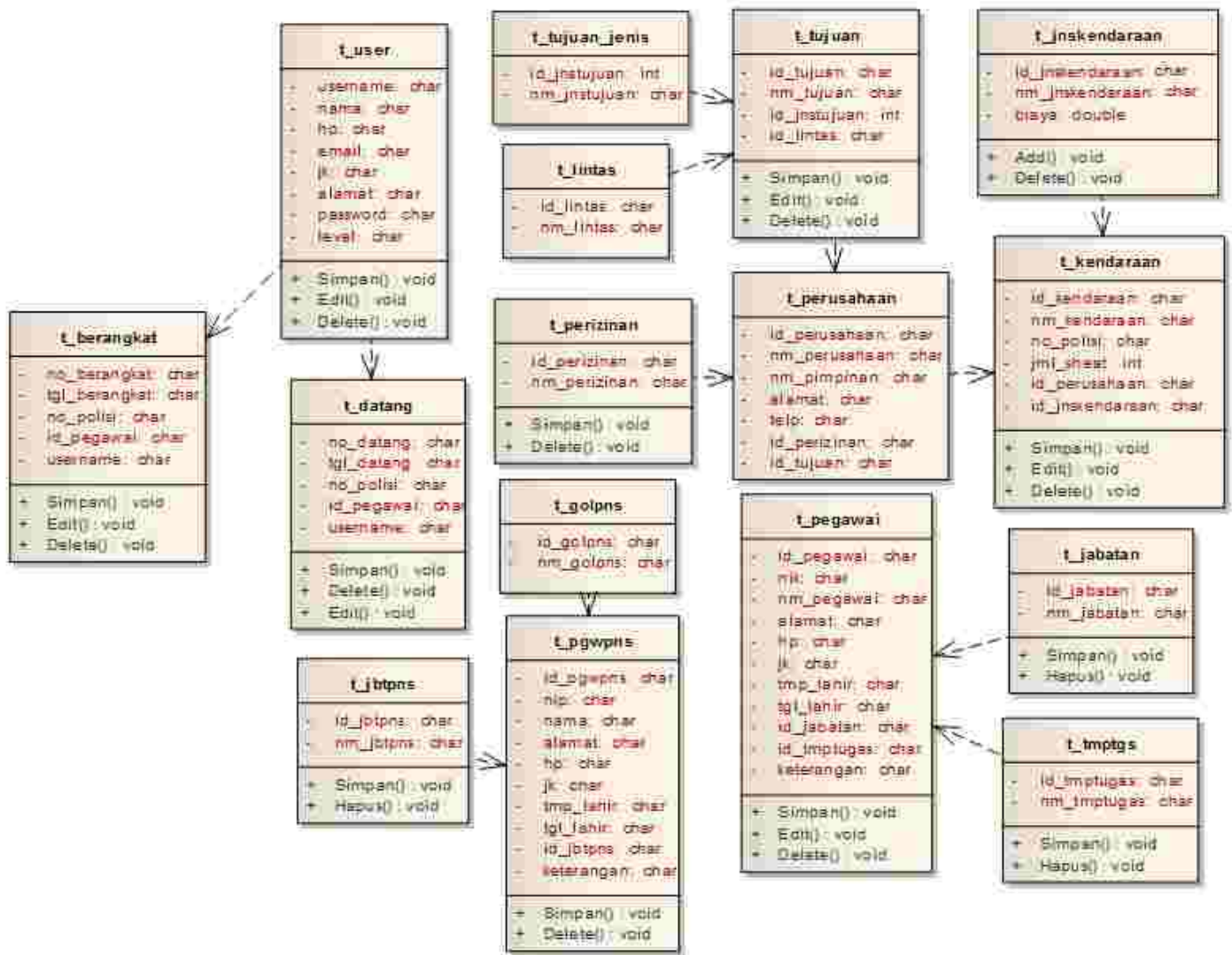
Gambar 5 : Class Diagram
