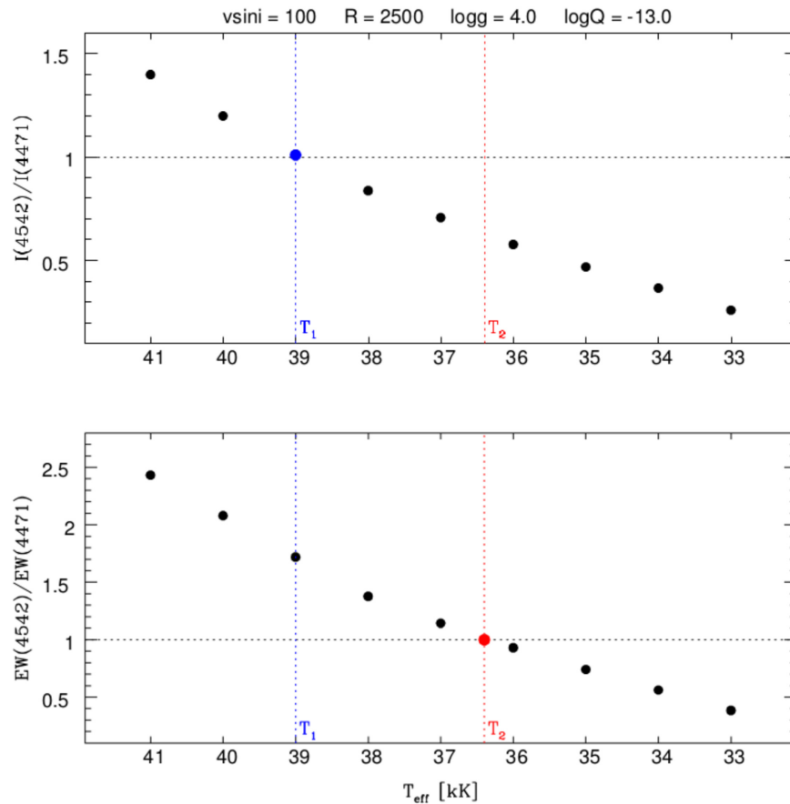
Figure 3. Top panel: variation of the ratio between the CDs of the He \text{I}\lambda 4471 and He \text{II}\lambda 4542 lines, as a function of T_{\text{eff}} , as shown by the FASTWIND model predictions. Bottom panel: the same for the ratio of EWs. Fixed values of the projected rotational velocity, surface gravity, resolution, and wind strength have been considered. T_1 and T_2 indicate the effective temperature suitable for the O7 spectral type when the latter is defined from the CDs or EWs ratios, respectively.
