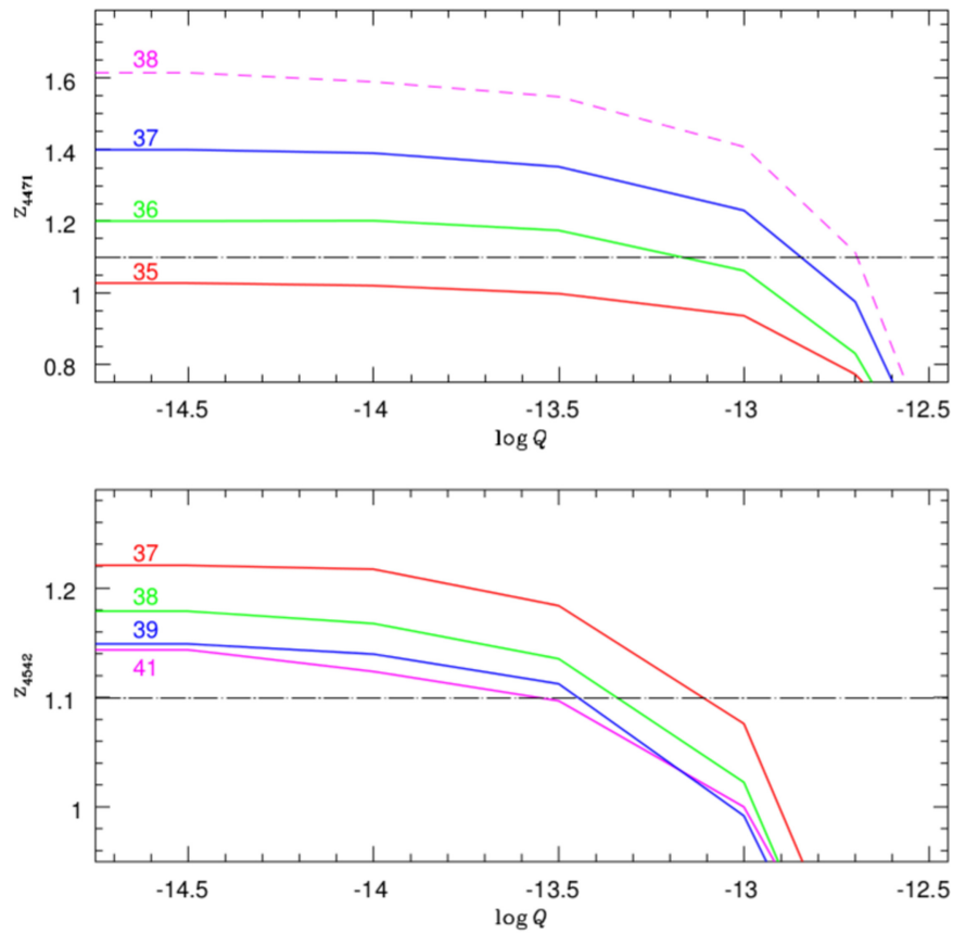
Figure 9. FASTWIND predictions of the behavior of the EW ratios that define the z spectral characteristic, with the variation of the wind-strength parameter Q . Fixed values of the resolution ( R = 2500 ), surface gravity ( \log g = 4.0 dex), and projected rotational velocity ( v \sin i = 100 \text{ km s}^{-1} ) have been considered. The labels next to each color curve indicate the corresponding effective temperature expressed in kK. In the upper panel, the dashed line for 38 kK indicates that this temperature is likely out of the z_{4471} relevant range.
