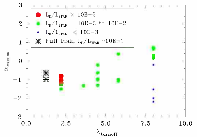
Figure 8. \alpha_{\text{excess}} vs. \lambda_{\text{turnoff}} for objects with different L_D/L_* values. The loci of “typical” CTTS with full disks are shown for comparison. Transition disks occupy a much larger parameter space.
