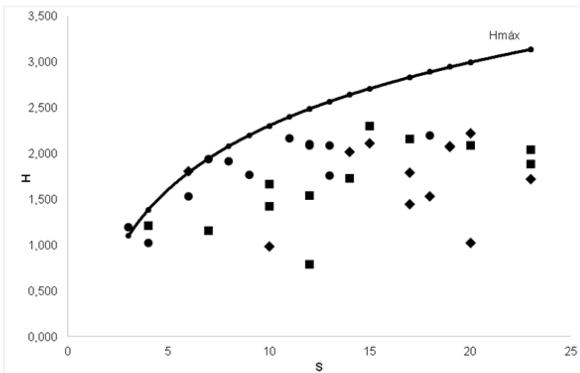
Figure 2. Diversity index ( H' ) in function with the number of taxa ( S ) for season 1 ●; season 2 ■ and season 3 ◆. Graph of the logarithmic curve of the maximum expected diversity ( H'max ).
