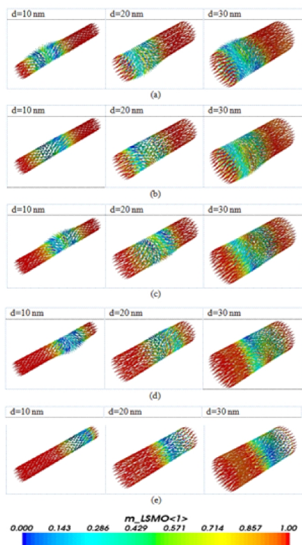
Figure 1. Evolution position domain wall in La_{1-x}Sr_xMnO_3(x=0,3) material with variations meeting current: (a) 1 \times 10^{10} \text{ A/m}^2 , (b) 2 \times 10^{10} \text{ A/m}^2 , (c) 4 \times 10^{10} \text{ A/m}^2 , (d) 6 \times 10^{10} \text{ A/m}^2 , (e) 8 \times 10^{10} \text{ A/m}^2 where each index color on the under side represented scala value magnetization
