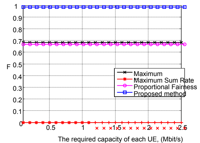
Fig. 2. Dependence of downlink channel bandwidth capacity balancing due to sub-channel allocation method used from the required bandwidth capacity
