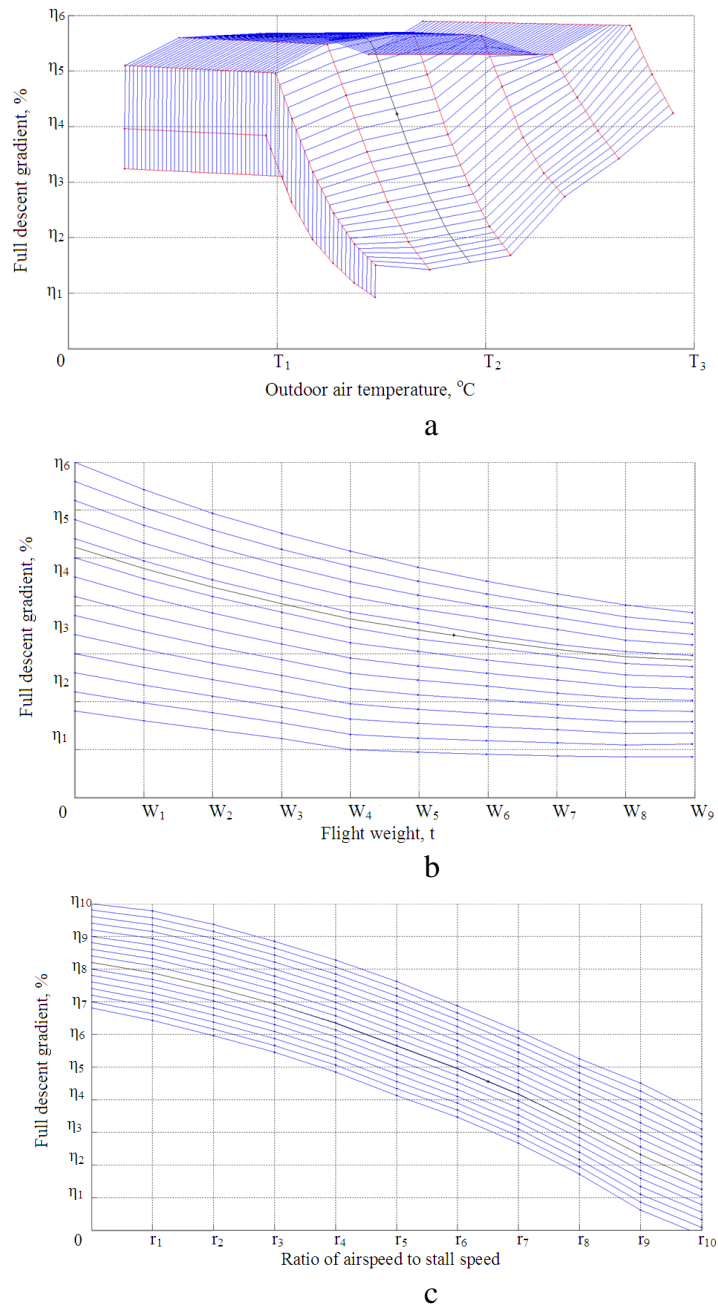
Fig. 1. Nomograms for determination of full descent gradient (thrust at idle): a) function of outdoor temperature ( T ), b) function of gross weight ( W ), c) function of ratio of airspeed to stall speed ( r )
