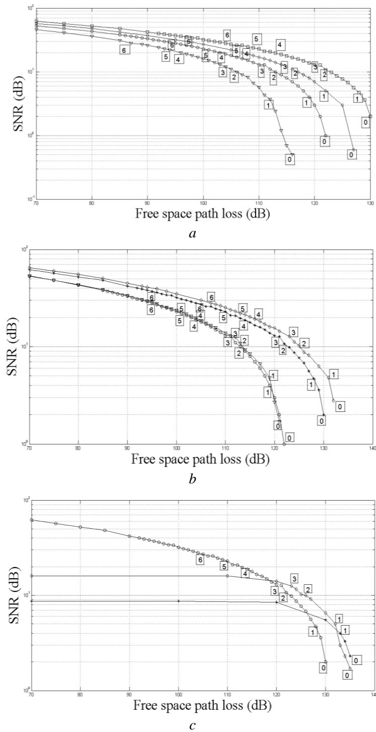
Fig. 2. The dependence of SNR on free space path loss in uplink/downlink for different types of modulation:
