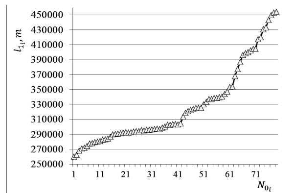
Fig. 1. Graph with a points of the distribution of values of model locations l_{1i} for n=1 for N_{0i} AVC
