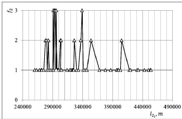
Fig. 6. The graph of the distribution of the class frequency f_2 for model location l_{2i} for n=2
