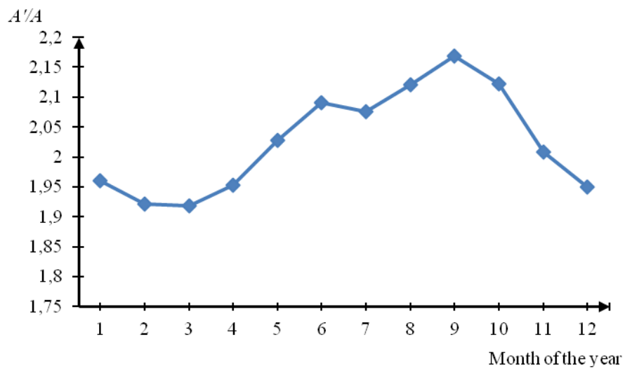
Fig. 3. Dependence of the area of additional cooling surface A' on time of the year
