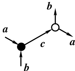
FIG. 1: The basic tile for the hexagonal lattice, showing the activities and our choice of Kastelyn orientation.
