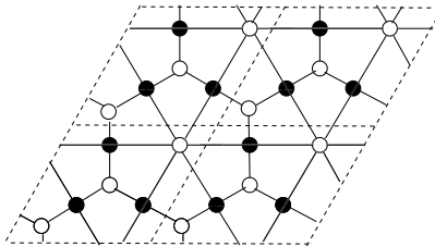
FIG. 2: Four copies of the basic tile for the tunable single oval model. For consistency we need to switch black and white and add an orientation plus activities.
