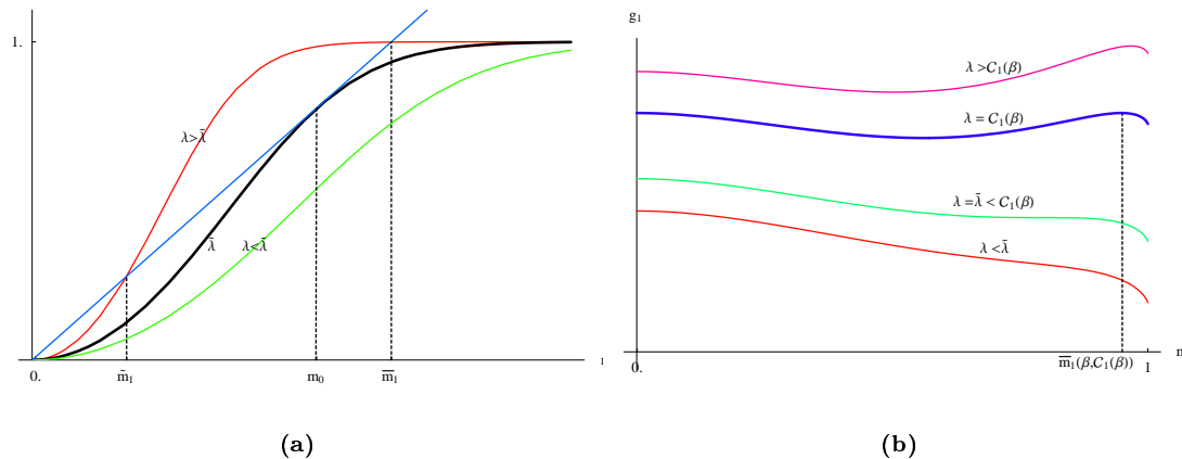
Figure 4.1: (a) \tanh[p\beta\lambda m^{p-1}] at \lambda \gtrless \tilde{\lambda} (b) \lambda = C_1(\beta) defines the critical value
