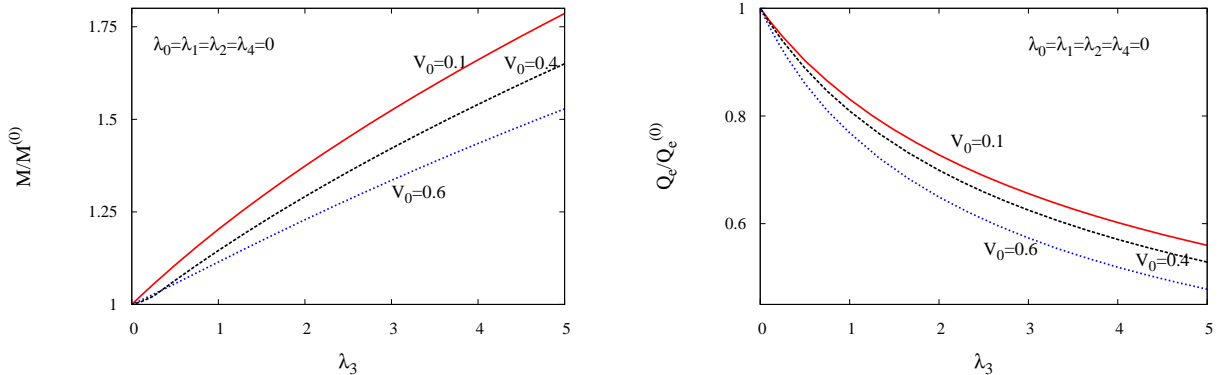
Figure 6. Same as Figure 4 for electrically charged, generalized dipole solutions.
