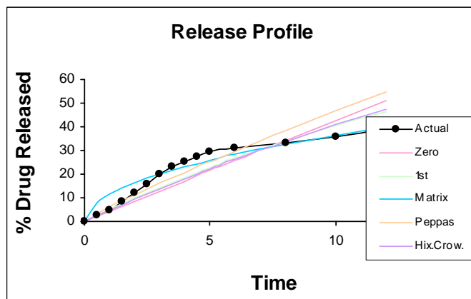
Fig. 2: Graph showing release kinetics of optimized formulation
