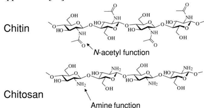
Figure 1. Structure of chitin and chitosan Emergence for New and Improved Vaccines
