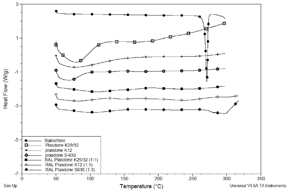
Figure 2. DSC of RHCL, Plasdone grades and Spray dried compositions
