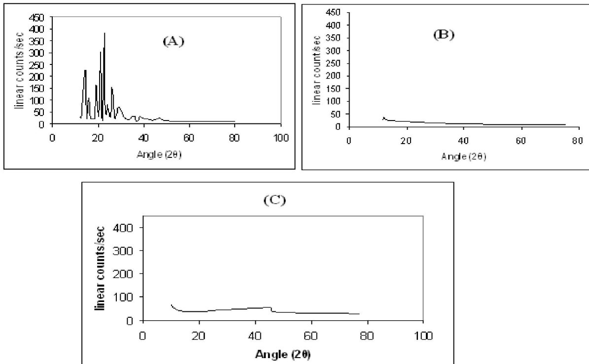
Figure 3. XRD Spectra of (A) RHCL; (B) PVP K12; (C) Spray dried RHCL : K12 1:1
