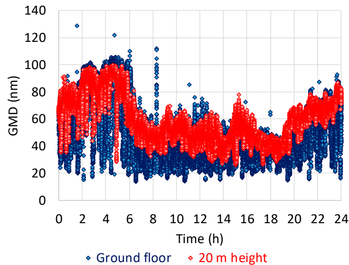
Figure 3. Temporal trend of the geometric mean aerodynamic diameter (GMD) at ground level and at 20 m height in a street canyon in downtown Rome.
