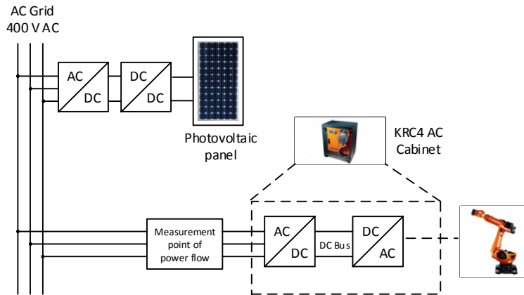
Fig. 1: Example of the state of the art AC supplied industrial robot system
