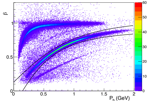
FIG. 4: (Color online) \beta versus momentum for positively charged protons. The solid lines show the cut used to select protons. The bands above the proton band are from K^+ , \pi^+ , and e^+/\mu^+ tracks, while deuterons are visible below the proton band. The color ( z ) axis represents the number of events.
