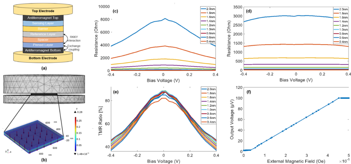
Fig.1 Schematic of the TMR stack layout used for FEM simulations.
