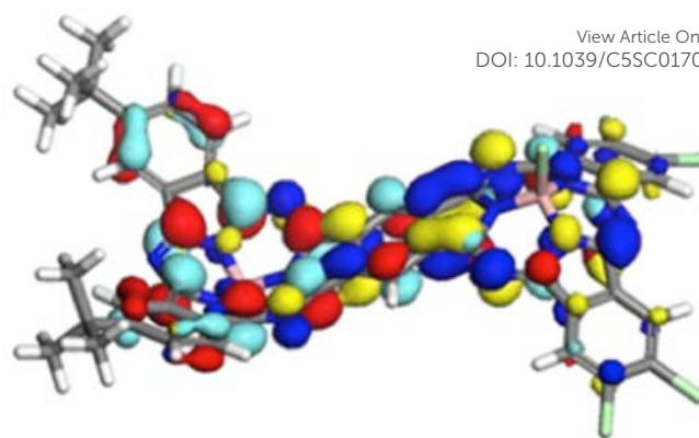
Fig. 5 HOMO (red/cyan) and LUMO (blue/yellow) of anti - 1 .
