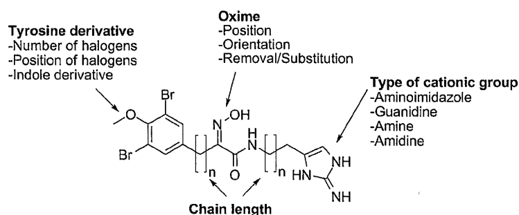
Fig. 5 Synthetic targets for structure activity relationship studies for establishing the AF pharmacophore of 1
