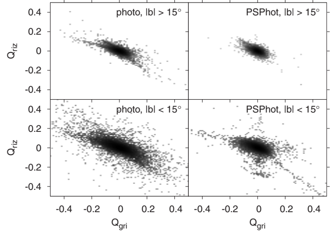
Figure 4. Distribution of median Q_{gri} - and Q_{riz} -parameters measuring the position of the stellar locus within each field for the photo (left) and PPShot (right) photometric pipelines; zero values are indicative of uniform photometry. Within the Galactic plane (lower panels), the PPShot values are more concentrated, but contain a higher number of systematic departures from the main locus. The PPShot code in fact gives a tighter locus at high latitudes as well (upper panels). Histogram equalization of the grayscale was used to emphasize low-density regions.
