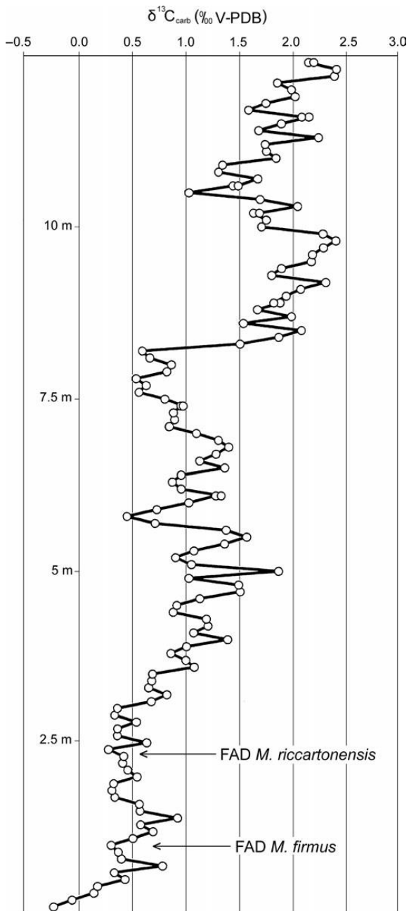
Fig. 2. The new \delta^{13}\text{C}_{\text{carb}} isotope curve through the measured lower Sheinwoodian section in Buttington Quarry, commencing in the Trevern Brook Mudstone Formation immediately above the top of the Butterley Member. First appearance datums of biozonal index graptolites are shown. Detailed sedimentological description of the section is at a preliminary stage: lithologies are grey mudrocks (shales and mudstones) throughout. For these reasons, no lithological log is provided.
