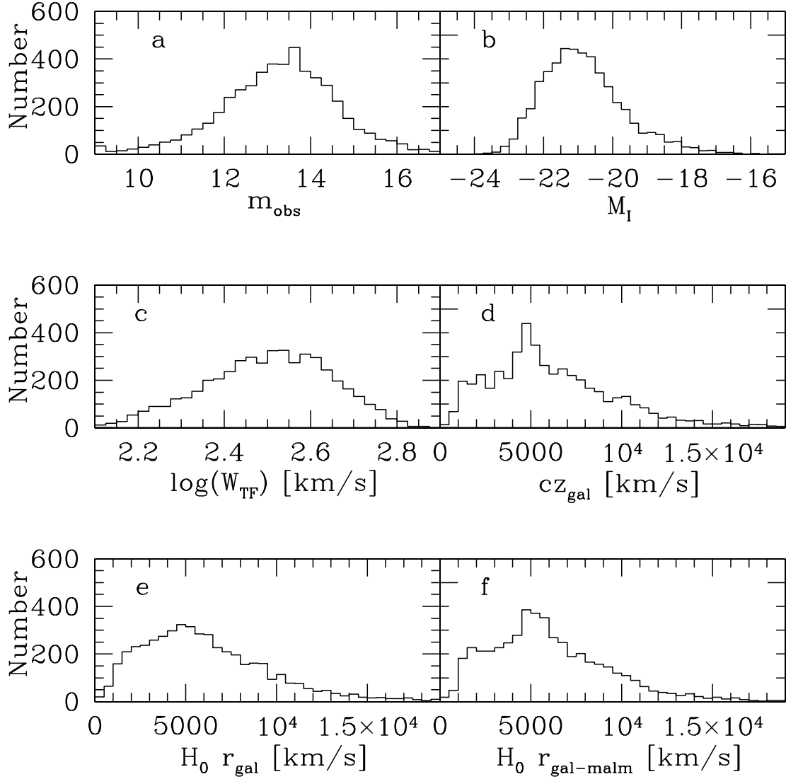
FIG. 4.—Distribution of (a) Observed I -band magnitude, in bins of width 0.25 mag; (b) I -band absolute magnitude, in bins of width 0.25 mag; (c) logarithm of velocity widths, in bins of width 0.025 dex, (d) recessional velocity in CMB frame, in bins of width 500 km s -1 ; (e) TF distance (uncorrected for Malmquist bias), in bins of width 500 km s -1 ; and (f) Malmquist bias-corrected TF distance, in bins of width 500 km s -1 , for all galaxies in the SFI++.
