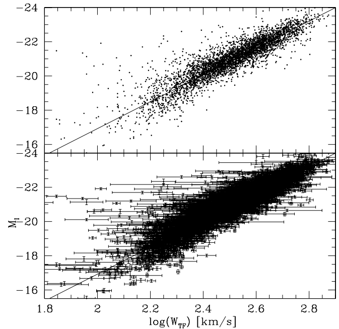
FIG. 6.— Top : TF relation for all nontemplate galaxies. Bottom : Same points plotted, but with magnitude and width error bars included. The solid line represents the template relation from Paper I, which we provide in eq. (14). The width-dependent morphological corrections of § 5 have been applied to the magnitudes plotted here, unlike the magnitudes in Table 2 and 4.
