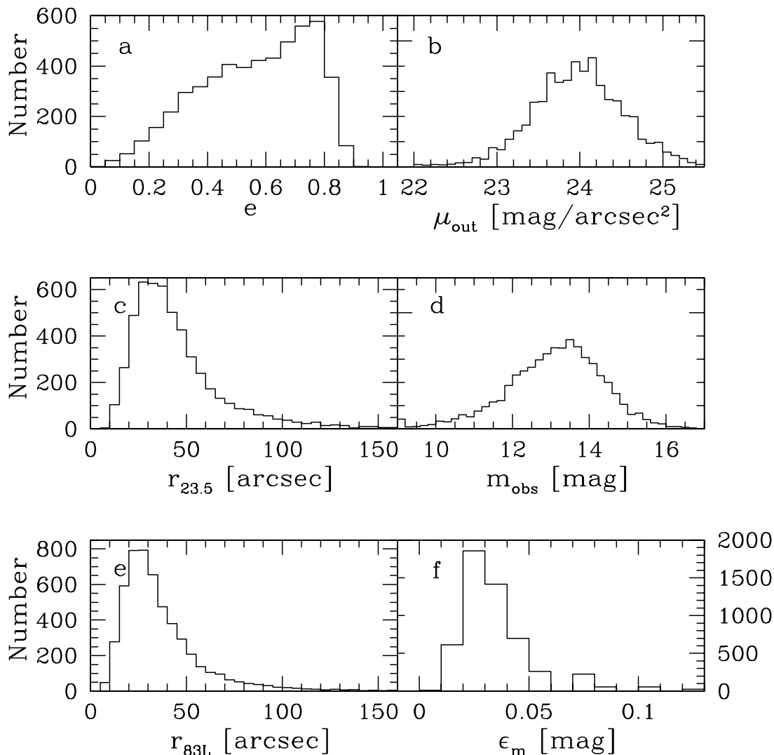
FIG. 1.—Distribution of (a) ellipticity, in bins of width 0.05; (b) surface magnitude at the outermost isophote, in bins of width 0.1 \text{ mag arcsec}^{-2} ; (c) isophotal radius at which the surface magnitude is 23.5 \text{ mag arcsec}^{-2} , in bins of width 5'' ; (d) observed I -band magnitude, in bins of width 0.2 \text{ mag} ; (e) optical radius encompassing 83% of the I -band light, in bins of width 5'' ; and (f) measurement error on the apparent I -band magnitude, in bins of width 0.01 \text{ mag} , for the 5254 galaxies for which we have these parameters. Note the difference in vertical scale between (e) and (f), in contrast to the identical vertical scales for the other adjacent pairs. Fig. 2 of H99 shows the distribution of the same parameters, albeit with some slightly different nomenclature, for the Sc sample that existed at that time.
