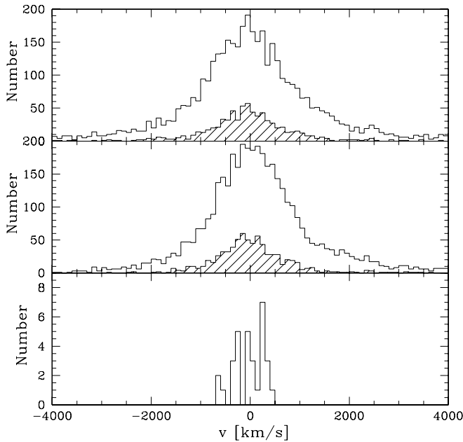
FIG. 5.— Top : Peculiar velocity distribution of all nontemplate groups ( hatched ) and all field galaxies ( unhatched ) before the Malmquist bias correction; middle : peculiar velocity distribution of all nontemplate groups ( hatched ) and all field galaxies ( unhatched ) after the Malmquist bias correction; bottom : peculiar velocity distribution of the template clusters. In all three plots, the bin width is 100 \text{ km s}^{-1} .
