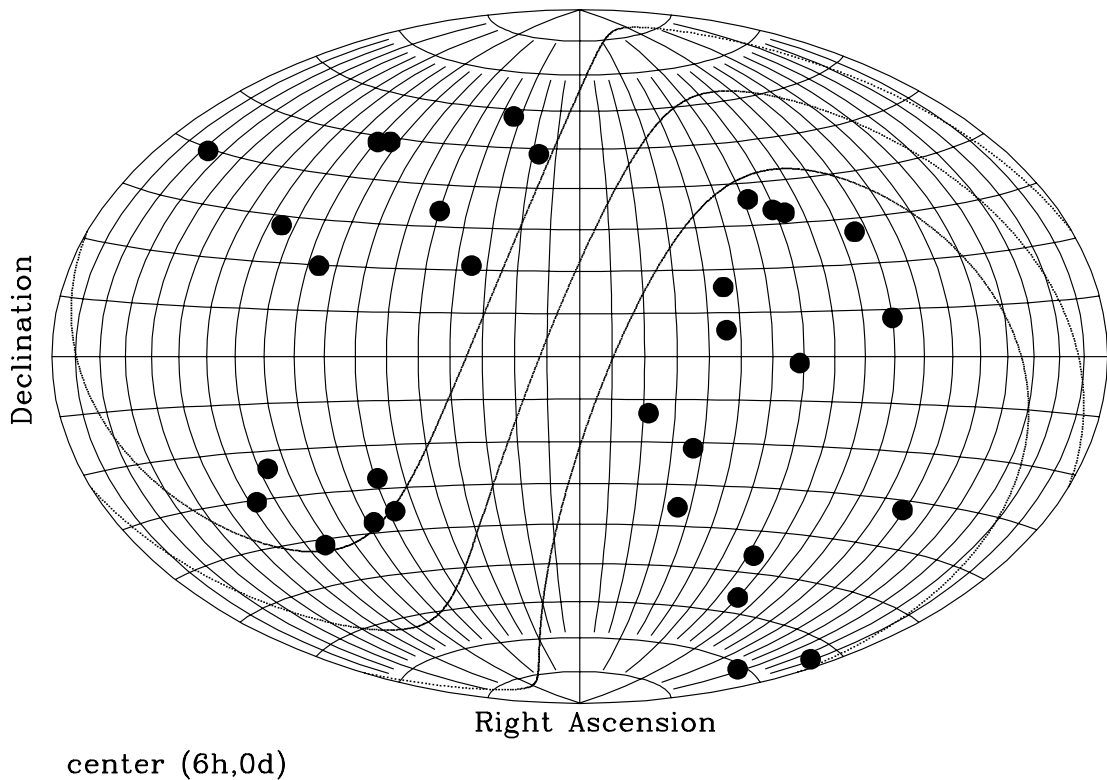
FIG. 3.—Same as Fig. 2, but for SFI++ template clusters. [See the electronic edition of the Supplement for a color version of this figure.]
