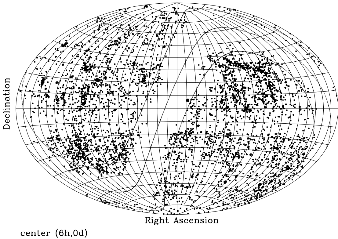
FIG. 2.—Aitoff equal area projection of the sky distribution of SFI++ galaxies. The plot is centered at R.A. = 6^{\text{h}} . The thick lines trace the Galactic latitudes b = -20^\circ , b = 0^\circ , and b = +20^\circ . [See the electronic edition of the Supplement for a color version of this figure.]
