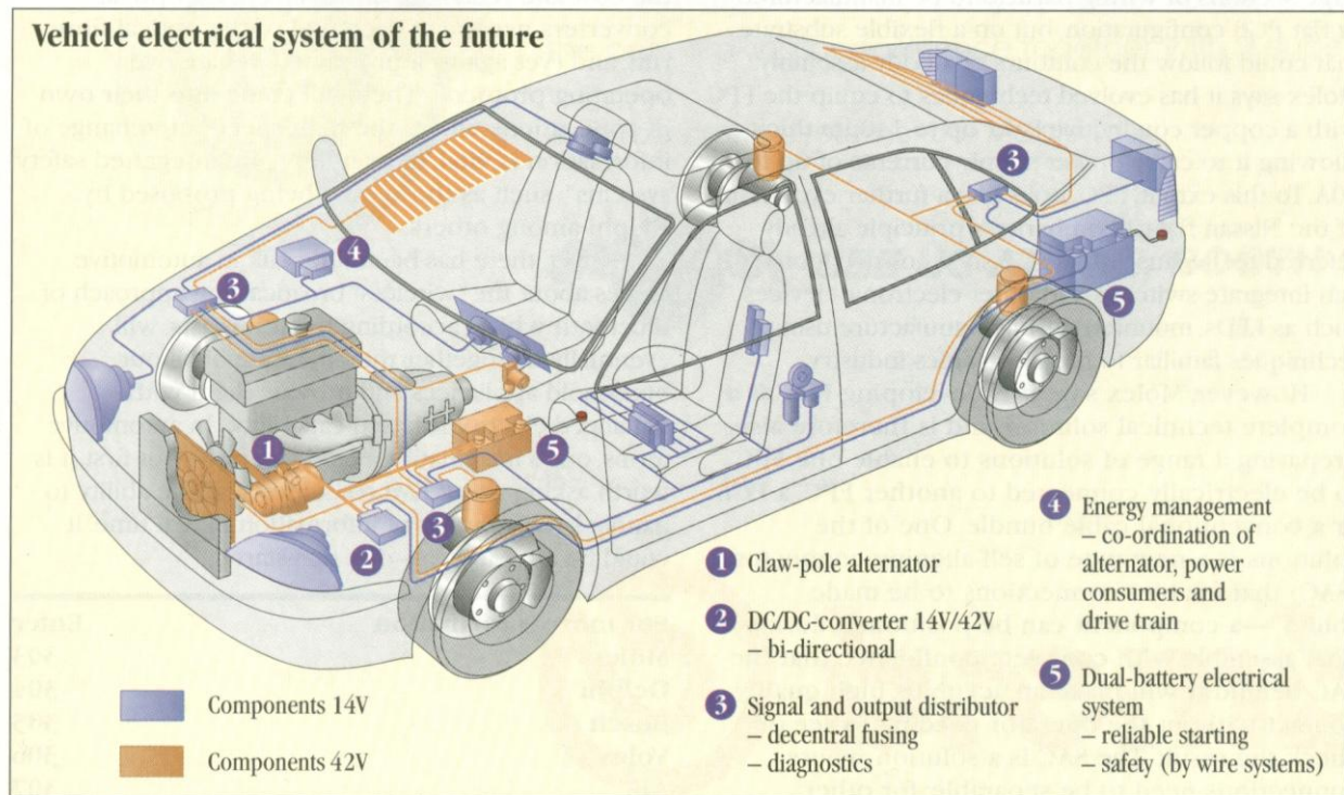
Figure 5: Vehicle electrical system of the future [Baldwin(2001)]
