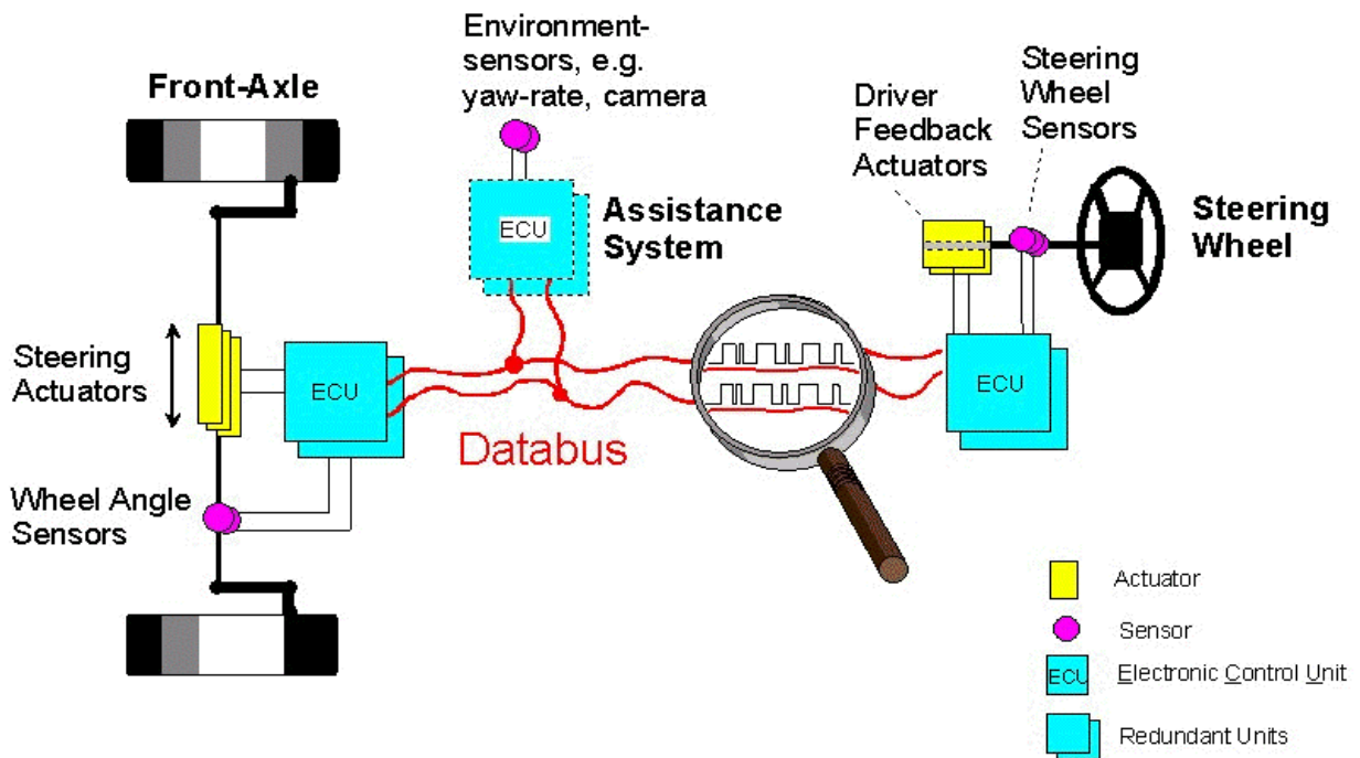
Figure 2: Steering system [From vmars xbywire project (2004)]
