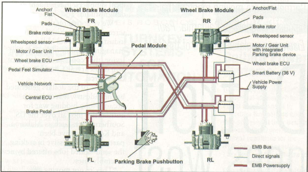
Figure 4: Electromechanical braking system [From Professional Engineering (2001)]
