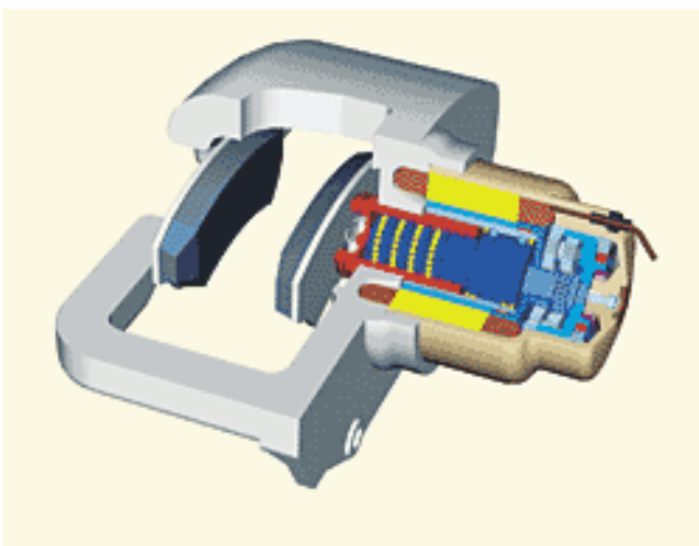
Figure 3: Electro mechanical brake calliper [From daimlerchrysler (2004)]
