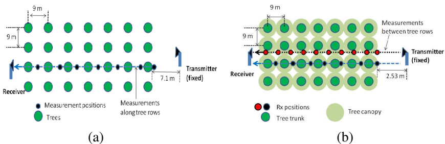
Figure 1. Vegetation geometry and measurement configurations: (a) mango plantation and, (b) palm plantation.
