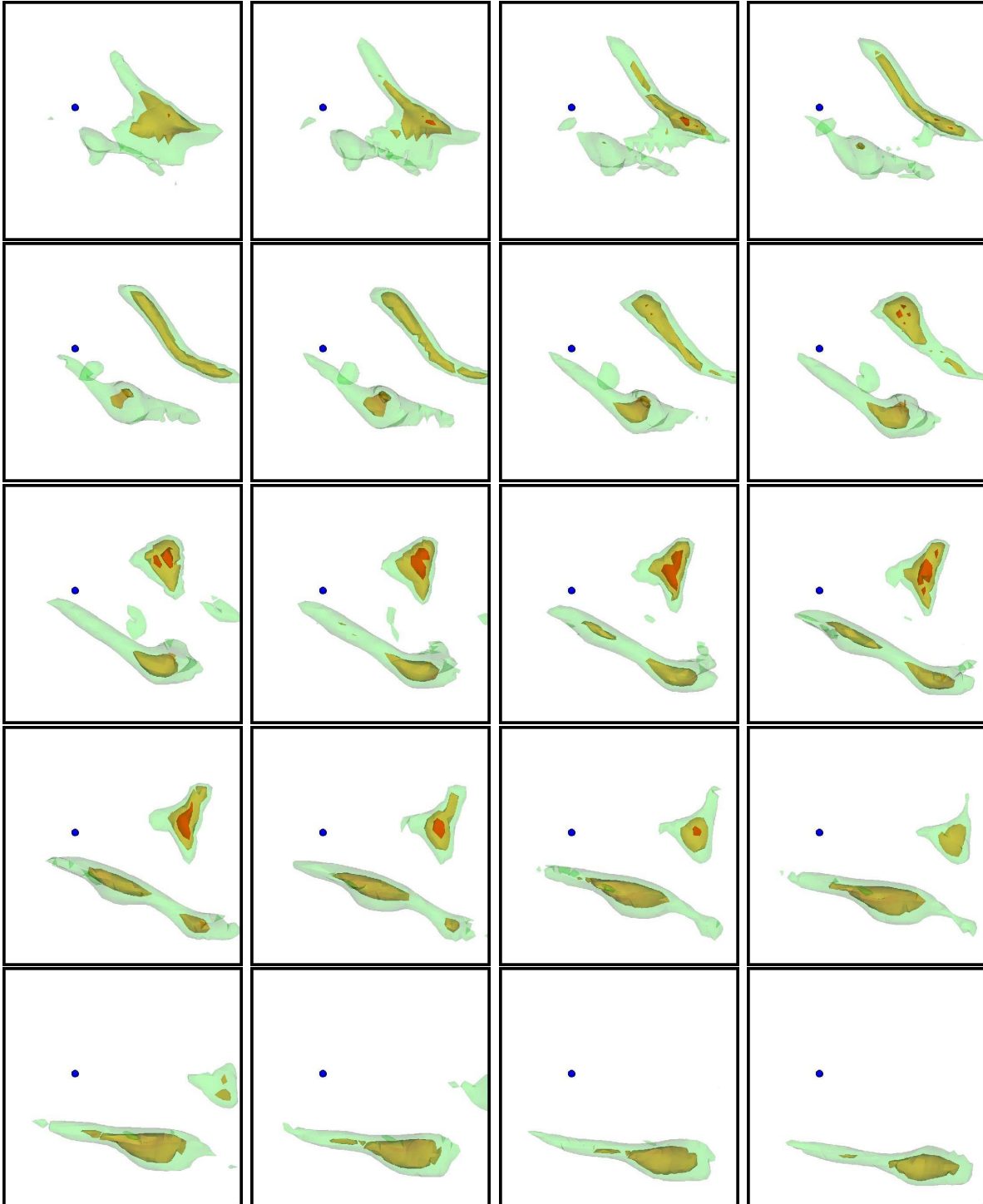
Fig. 13.— Temperature contours from t = 10454.6 s to t = 10458.4 s (corresponding to the blue dotted time range in Figure 11) spaced at 0.2 s time intervals. The contours are surfaces indicating where T = 7.24 \times 10^8 K (green), T = 7.31 \times 10^8 K (yellow), and T = 7.38 \times 10^8 K (orange). The blue dot is at the center of the star, and has a diameter of 4.34 km, which corresponds to the grid cell width for this simulation.
