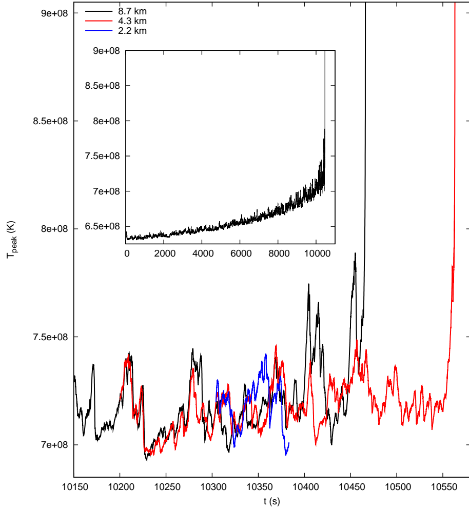
Fig. 3.— Peak temperature leading up to ignition for the 8.68 km, 4.34 km, and 2.17 km simulations. The inset plot shows the long-time behavior of the 8.68 km simulation originally presented in Z11.
