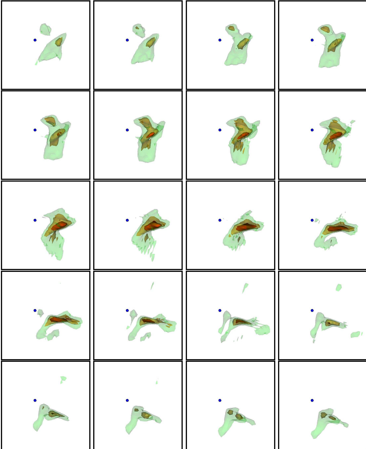
Fig. 12.— Temperature contours from t = 10404.0 s to t = 10407.8 s (corresponding to the green dotted time range in Figure 11) spaced at 0.2 s time intervals. The contours are surfaces indicating where T = 7.15 \times 10^8 K (green), T = 7.2 \times 10^8 K (yellow), and T = 7.25 \times 10^8 K (orange). The blue dot is at the center of the star, and has a diameter of 4.34 km, which corresponds to the grid cell width for this simulation.
