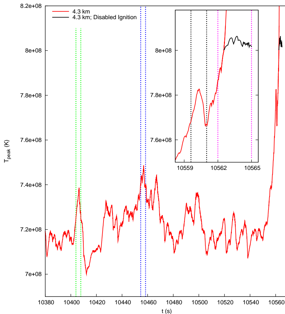
Fig. 11.— Peak temperature during the \sim 200 s preceding ignition for the 4.34 km simulation. The dashed vertical lines indicate time ranges where we will examine whether there are multiple hot spots. The inset plot is a zoom-in of the final \sim 5 s preceding ignition. The black curve follows the maximum temperature for a simulation where we disable burning in all cells with T > 8 \times 10^8 K.
