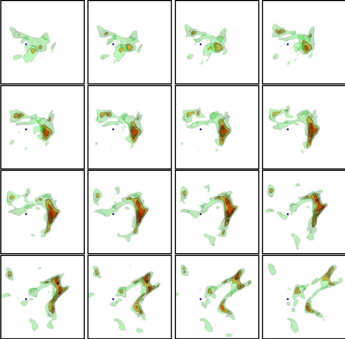
Fig. 15.— Temperature contours from t = 10562.0 s to t = 10565.0 s (corresponding to the pink dotted time range in Figure 11) spaced at 0.2 s time intervals. The contours are surfaces indicating where T = 7.5 \times 10^8 K (green), T = 7.7 \times 10^8 K (yellow), and T = 7.9 \times 10^8 K (orange). The blue dot is at the center of the star, and has a diameter of 4.34 km, which corresponds to the grid cell width for this simulation.
