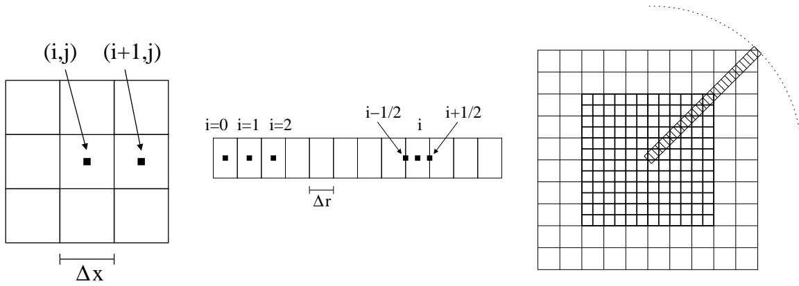
Fig. 1.— (Left) For data on the Cartesian grid (shown here in two dimensions), we use a cell-centered convention to denote the average value over the computational cell. (Center) The base state variables live on a one-dimensional radial array, and can live at cell centers or edges. (Right) A graphical depiction of how the base state and Cartesian grid are related. Note that there is no direct alignment between the radial cell centers and the Cartesian grid cell centers.
