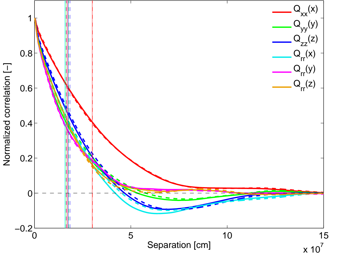
Fig. 21.— Longitudinal correlation functions for the turbulence in the convective core at 2.17 km resolution for t = 10380 . Density-weighted and non-weighted correlation functions are shown by solid and dashed lines, respectively. The x component presents a larger correlation because there is a plume-like structure roughly aligned with the x -axis. The integral length scales are denoted by the vertical lines of the corresponding color.
