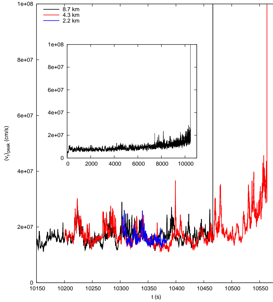
Fig. 5.— Peak radial velocity leading up to ignition for the 8.68 km, 4.34 km, and 2.17 km simulations. The inset plot shows the long-time behavior of the 8.68 km simulation originally presented in Z11.
