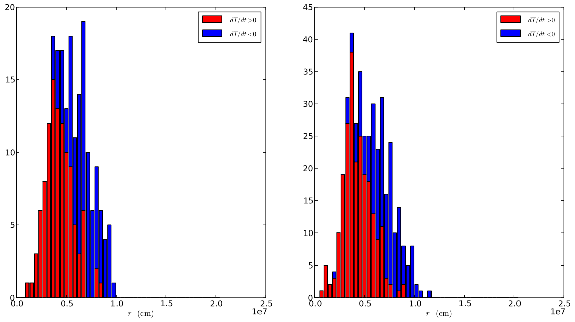
Fig. 10.— Histograms of the hottest cell, sorted by radius, with the colors indicating whether the temperature of the hottest cell is increasing or decreasing with time for the 4.34 km simulation with (Left) \Delta t_{\text{hist}} = 1.0 s and (Right) \Delta t_{\text{hist}} = 0.5 s.
