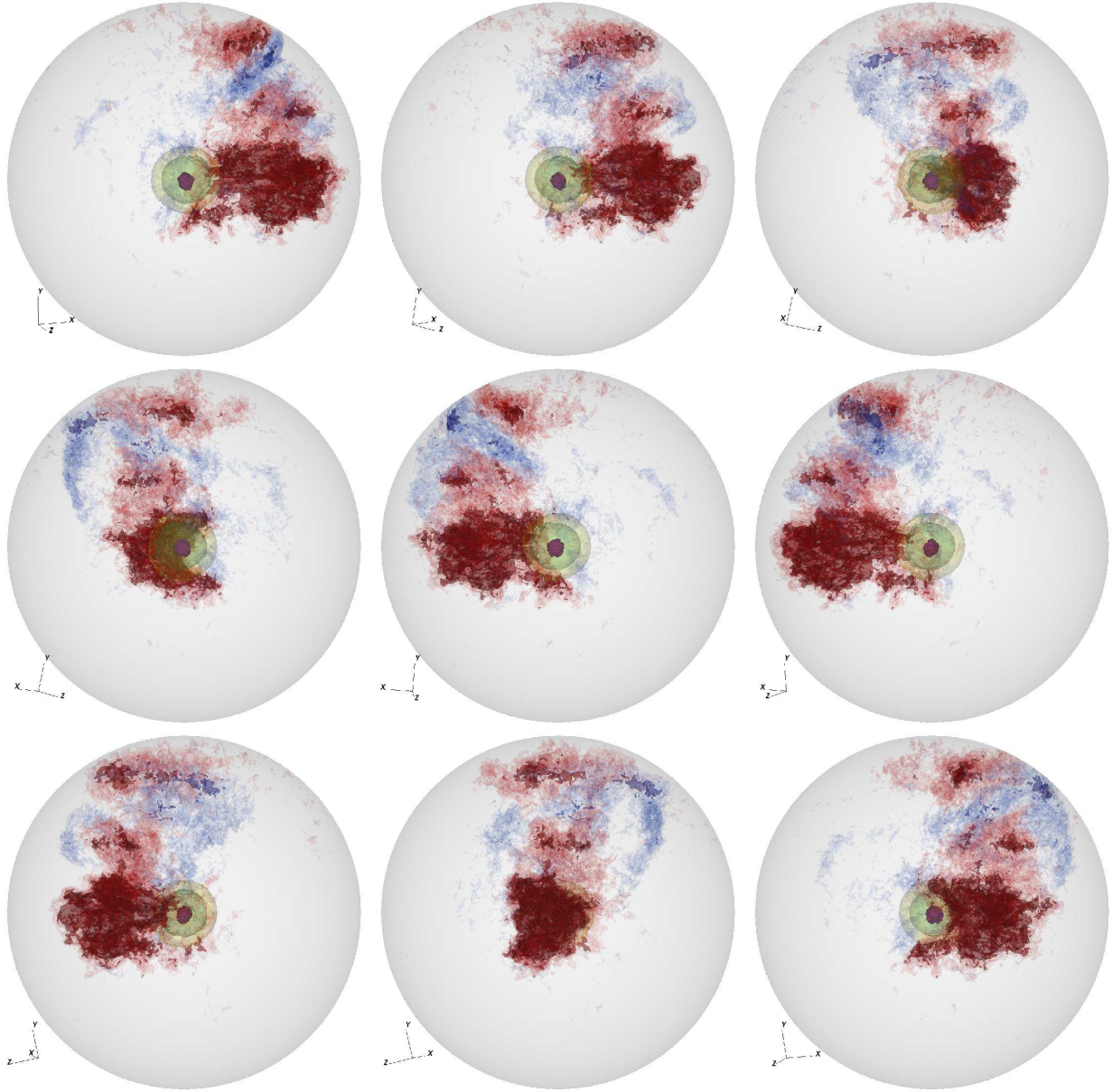
Fig. 17.— Same data as Figure 16, but here we only show the 2.17 km grid cell simulation, and each image represents a view rotation of 40 degrees of the data from t=10380 s.
