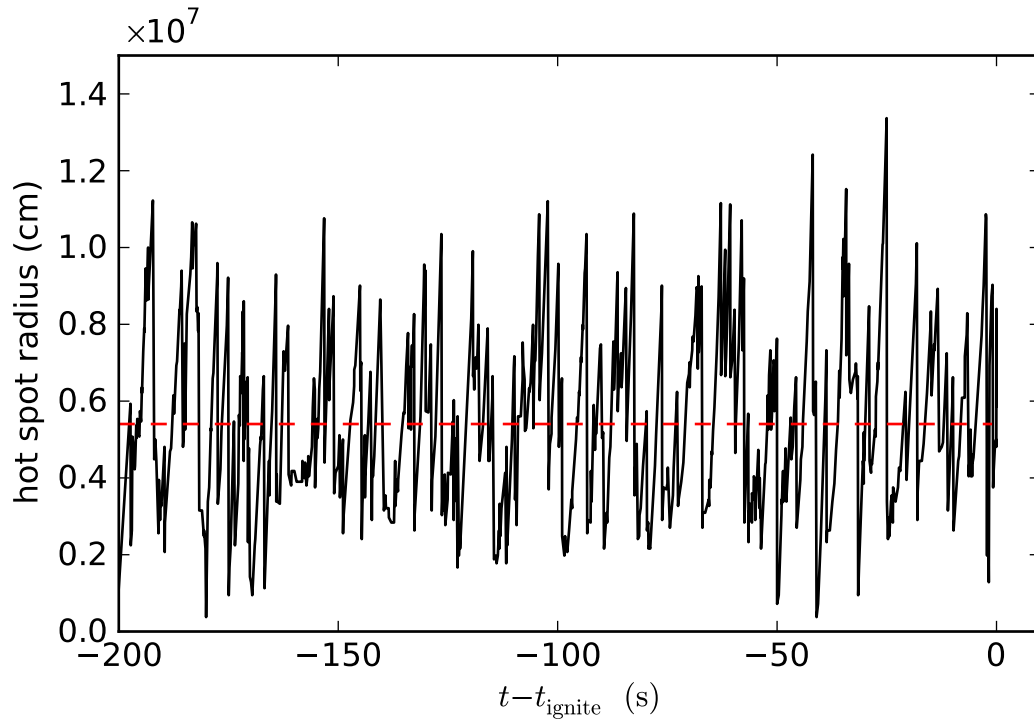
Fig. 6.— Radial location of the hottest cell as a function of time for the 4.34 km simulation. Only the last 200 s before ignition are shown. Here we see that right up to the end of the calculation the hot spot location changes rapidly. The horizontal horizontal dashed line indicates the average radial position of the hot spot from 200 s to 1 s before ignition.
