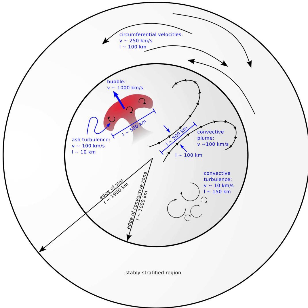
Fig. 22.— Cartoon showing the various features with associated velocities and length scales in the white dwarf at the end of convection/start of flame propagation.
