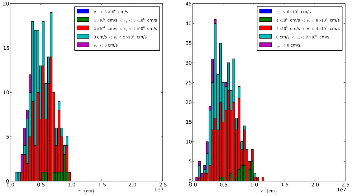
Fig. 8.— Histograms of the hottest cell, sorted by radius, with the colors representing the average radial velocity of the hottest cell over the averaging interval for the 4.34 km simulation with (Left) \Delta t_{\text{hist}} = 1.0 s and (Right) \Delta t_{\text{hist}} = 0.5 s.
