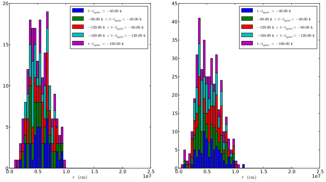
Fig. 9.— Histograms of the hottest cell, sorted by radius, with the colors representing time to ignition for the 4.34 km simulation with (Left) \Delta t_{\text{hist}} = 1.0 s and (Right) \Delta t_{\text{hist}} = 0.5 s.
