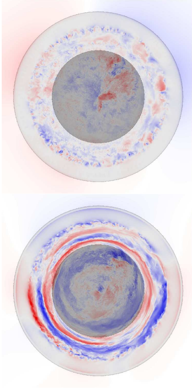
Fig. 19.— (Top) Plot of radial velocity ( \mathbf{U} \cdot \mathbf{e}_r ) in the x - y plane from the 2.17 km simulation at t = 10380 s. (Bottom) Plot of \mathbf{U} \cdot \mathbf{e}_\theta in the x - y plane from the same dataset. In both plots, red = +100 \text{ km s}^{-1} and blue = -100 \text{ km s}^{-1} . The outer dark contour indicates the edge of the star, where \rho_0 \approx 1 \times 10^5 \text{ g cm}^{-3} ( r \approx 1030 \text{ km} ). The inner dark contour indicates the edge of the convective region, where \rho_0 \approx 1.26 \times 10^8 \text{ g cm}^{-3} ( r \approx 1890 \text{ km} ).
