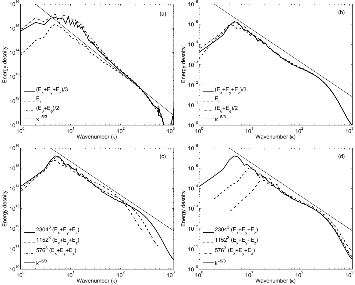
Fig. 20.— (a) Energy density spectra of the entire domain at 2.17 km resolution for t = 10380 . Note how the radial spectrum is much lower than the other components. This is due to the large circumferential velocities outside the convective core. (b) Energy density spectra for the convective core. Note how the curves have collapsed to a single profile, especially for \kappa \gtrsim 20 , corresponding to about 250 km. (c) Comparison of the energy density spectra at the three different resolutions. (d) As (c), but scaled to demonstrate that the effective Kolmogorov length scale is proportional to the computational cell width.
