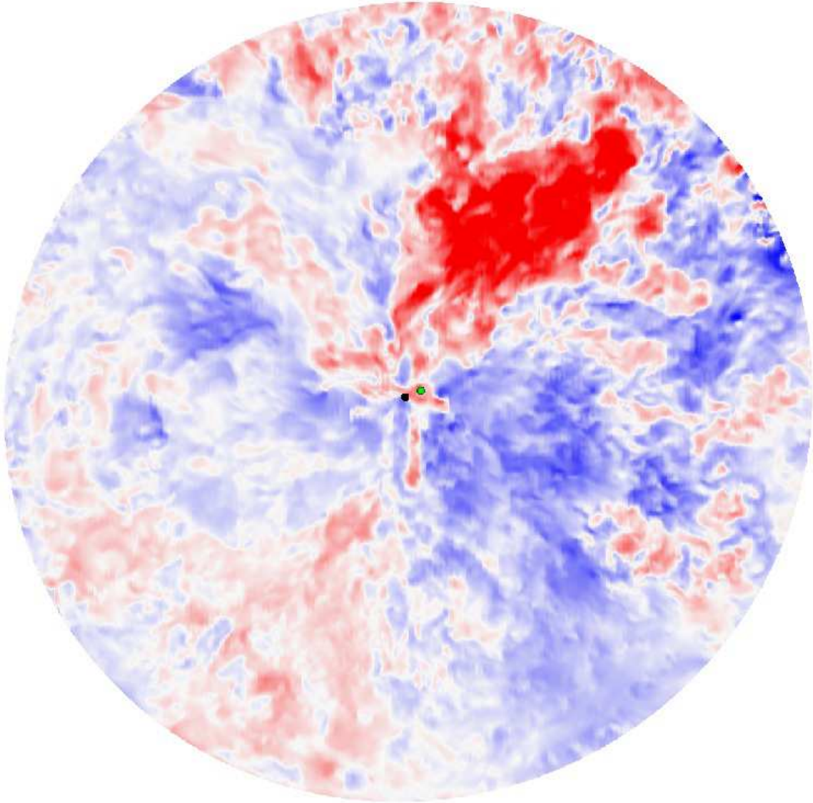
Fig. 18.— Planar slice from the 4.34 km simulation at the time of ignition, oriented so the center of the star (black dot), the ignition location (green dot), and the center of the strongest outward plume lie in the plane. The dots each have a radius of 20 km. Red corresponds to v_r > 60 \text{ km s}^{-1} and blue corresponds to v_r < -60 \text{ km s}^{-1} . Only the inner r = 1000 \text{ km} is shown.
