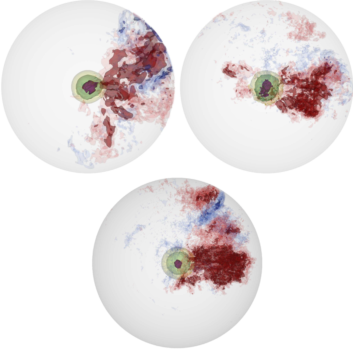
Fig. 16.— Contours of nuclear energy generation rate (yellow to green to purple, corresponding to 4 \times 10^{12} , 1.27 \times 10^{13} , and 4 \times 10^{13} \text{erg g}^{-1} \text{s}^{-1} ) and radial velocity (red is outflow, corresponding to 3 \times 10^6 and 6 \times 10^6 \text{cm s}^{-1} ; blue is inflow, corresponding to -3 \times 10^6 and -6 \times 10^6 \text{cm s}^{-1} ) for the (clockwise, from top-left) 8.68 km, 4.34 km, and 2.17 km simulations at t=10380 s. Only the inner r = 1000 km are shown.
