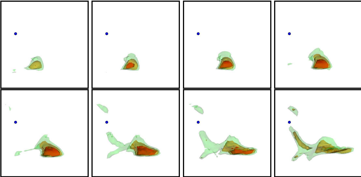
Fig. 14.— Temperature contours from t = 10559.2 s to t = 10560.6 s (corresponding to the black dotted time range in Figure 11) spaced at 0.2 s time intervals. The contours are surfaces indicating where T = 7.48 \times 10^8 K (green), T = 7.54 \times 10^8 K (yellow), and T = 7.6 \times 10^8 K (orange). The blue dot is at the center of the star, and has a diameter of 4.34 km, which corresponds to the grid cell width for this simulation.
