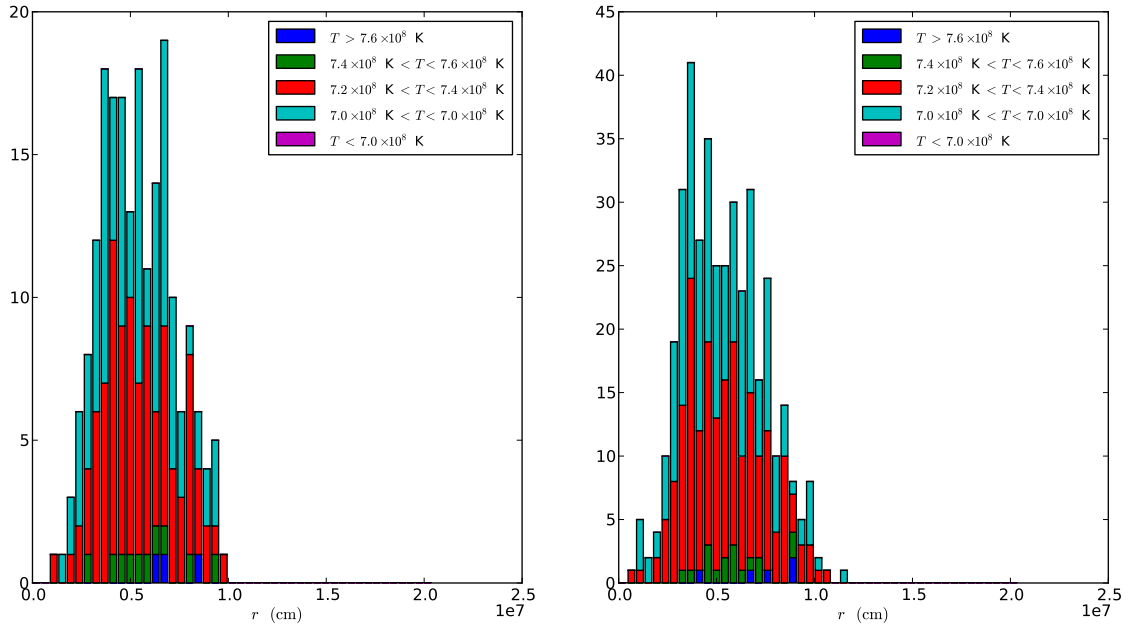
Fig. 7.— Histograms of the hottest cell, sorted by radius, with the colors representing the average temperature of the hottest cell over the averaging interval for the 4.34 km simulation with (Left) \Delta t_{\text{hist}} = 1.0 s and (Right) \Delta t_{\text{hist}} = 0.5 s.
