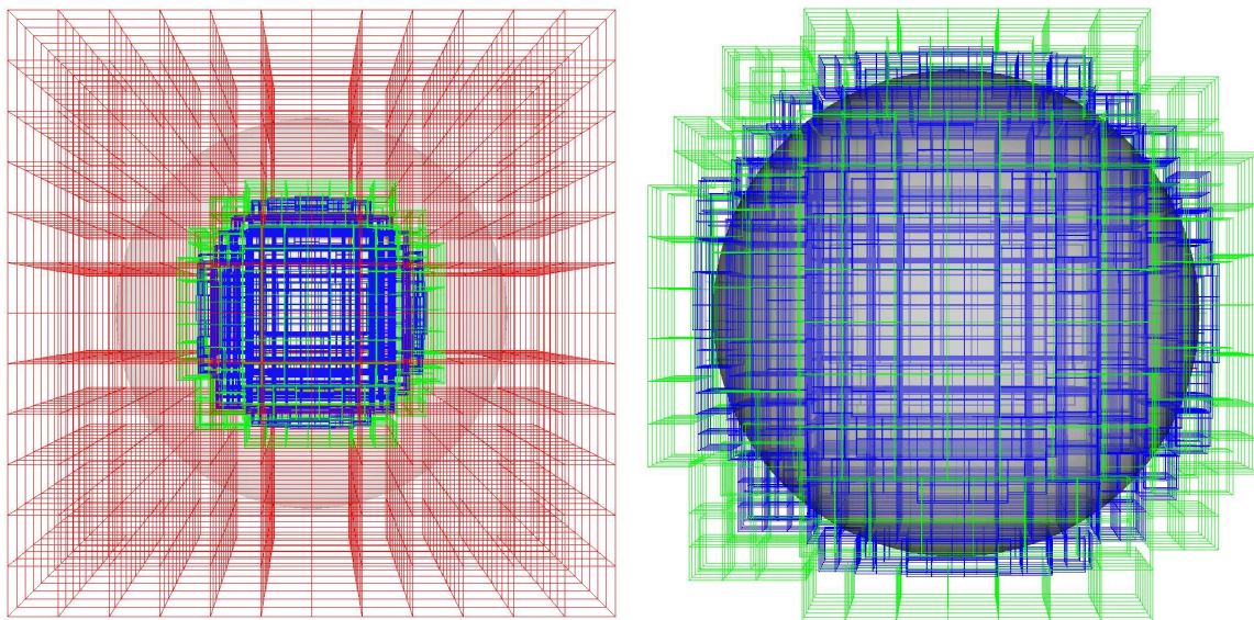
Fig. 2.— Grid structure for our three-level simulations. The base grid has 576^3 grid cells (8.68 km resolution), and the refined grids have effective 1152^3 (4.34 km) and 2304^3 (2.17 km) grid cells. The red, green, and blue outlines indicate boxes which can contain up to 64^3 grid cells. (Left) The shaded region indicates the edge of the star, defined by the location where \rho = 10^5 \text{ g cm}^{-3} at r \approx 1890 \text{ km} . (Right) In this zoom-in, the shaded region indicates the edge of the convective region, defined by the location where \rho \approx 1.26 \times 10^8 \text{ g cm}^{-3} at r \approx 1030 \text{ km} . The finest grids contain the entire convective region.
