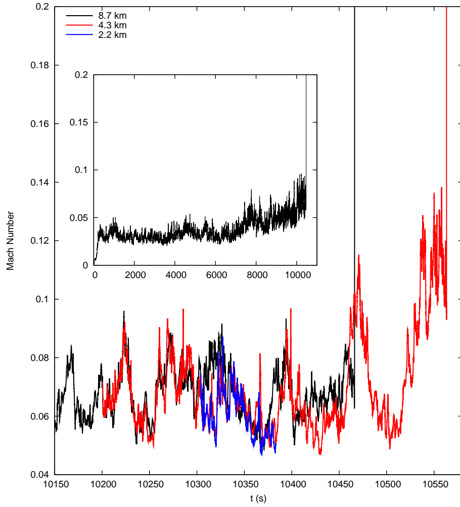
Fig. 4.— Peak Mach number leading up to ignition for the 8.68 km, 4.34 km, and 2.17 km simulations. The inset plot shows the long-time behavior of the 8.68 km simulation originally presented in Z11.
