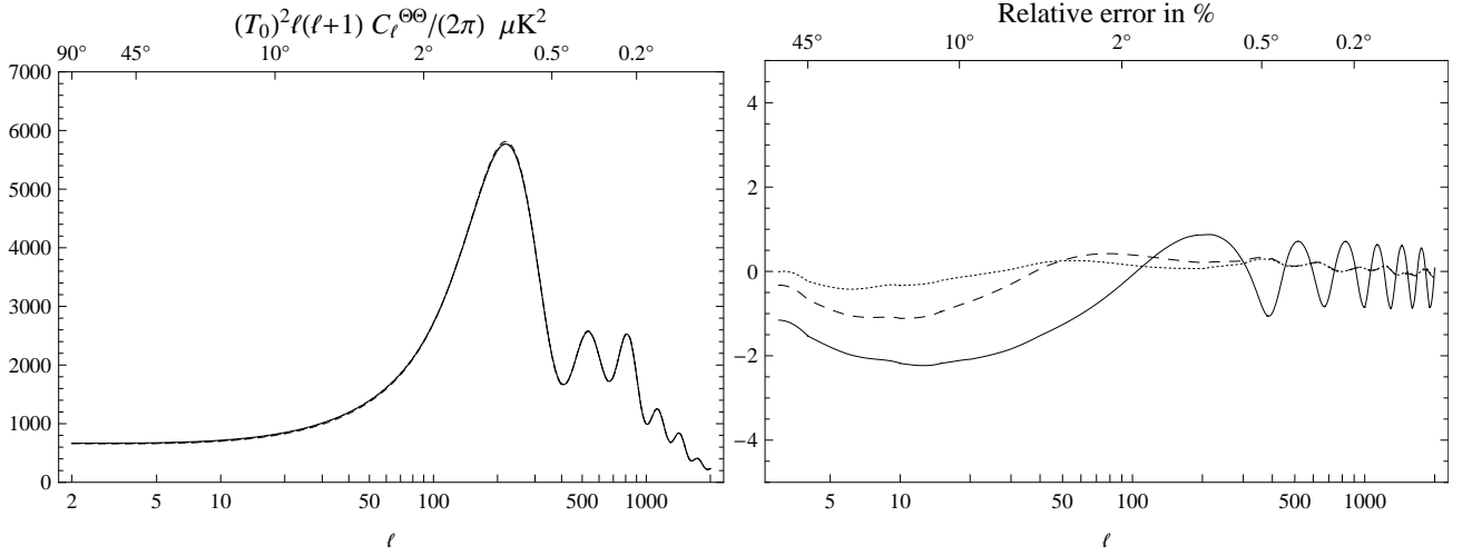
FIG. 4: Left : Comparison of the flat-sky approximations with the constraint k_{\perp} r = \sqrt{\ell(\ell+1)} while including only the lowest order in the expression (53) (dashed line) or adding its correction of order \ell^{-1} (dotted line) to the exact computation (solid line, standard cosmology, ignoring only the late time ISW effect). The calculations in the flat-sky approximations have been done using the thin-shell approximation.
