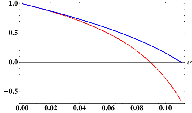
FIG. 2: A_{\dot{Q}_3^2} in Eq. (4.11) (dashed red) and A_{\dot{Q}_\sigma(\partial Q_\sigma)^2} in Eq. (4.12) (plain blue) as we vary \alpha with c_{\mathcal{D}}^2 \ll 1 .
