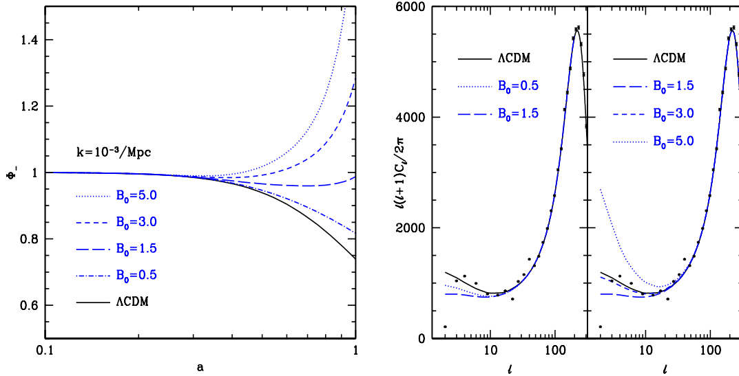
FIG. 3: Left : The ISW potential, (\Phi - \Psi)/2 , for f(R) models, where the parameter B_0 indicates the strength of deviation from general relativity [see Eq. (43)]. Right : The large-angle CMB anisotropies for the models of the left figure. (For more details see [43], where this figure is taken from.)
