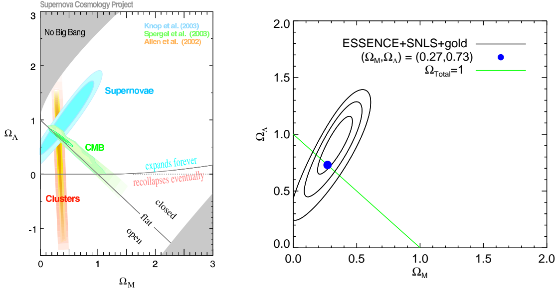
Fig. 1. Observational constraints in the (\Omega_{(m)}, \Omega_\Lambda) plane: joint constraints (left) (from [17]); recent compilation of supernova constraints (right) (from [18]).
