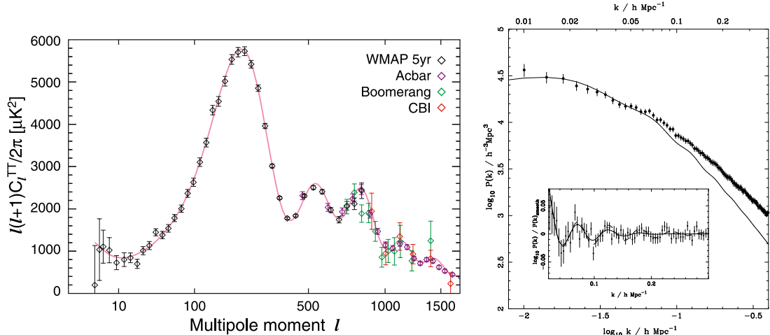
Fig. 2. Left: Power spectrum of CMB temperature anisotropies, showing data from WMAP5 [19], the 2003 flight of BOOMERANG [20], CBI [21] and the full ACBAR dataset [22]. The red line is the best-fit LCDM model to the data. Right: Matter power spectrum, showing data from the SDSS 2006 data release and the best-fit LCDM curve; the inset shows the imprint (in Fourier space) of the CMB acoustic peaks, known as the baryon acoustic oscillations (from [2]).
