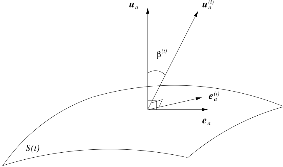
Fig. 3. In a multi-component system, the 4-velocity u_a^{(i)} of the i -th fluid makes a hyperbolic angle \beta^{(i)} with the fundamental 4-velocity field u_a , normal to the hypersurfaces of homogeneity S(t) . The unit vectors e_a and e_a^{(i)} are orthogonal to u_a and u_a^{(i)} respectively. Following definition (2.4.2), the peculiar velocity of the i -th species is v_a^{(i)} = v^{(i)}e_a , with v_{(i)}^2 = v_a^{(i)}v_a^{(i)} .
