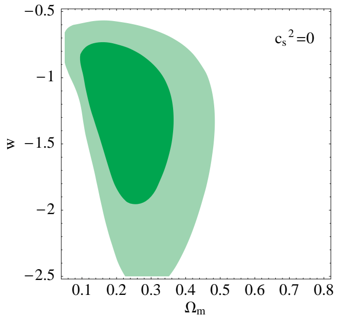
FIG. 11: Likelihood for flat models with varying \Omega_m and w from the MC2 errors. The shaded areas represent 1 and 2 \sigma intervals. The top panel assumes relativistic sound speed, such as would occur in a quintessence model, while the lower panel assumes the opposite extreme of zero sound speed.
