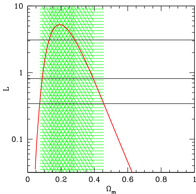
FIG. 10: Likelihood for flat models with varying \Omega_m from the MC1 and MC2 errors. The shaded areas represent 1, 2 and 3 \sigma intervals for \Omega_m . \Lambda CDM is a good fit to the data.
