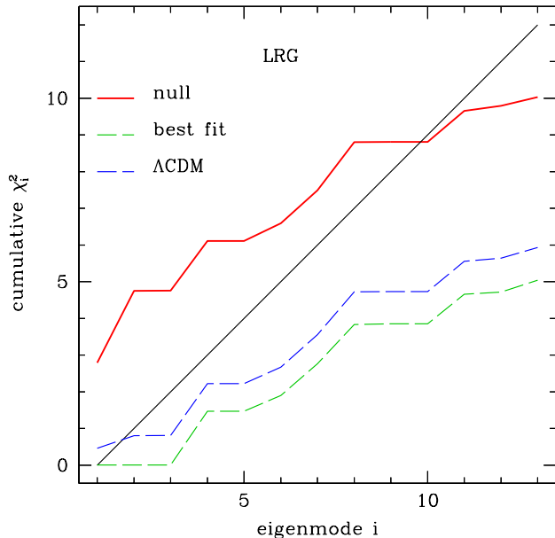
FIG. 9: Cumulative \chi_i^2 obtained summing the contribution up to the i -th eigenmode, for the three models: null hypothesis (red solid), best fit and \Lambda CDM .
