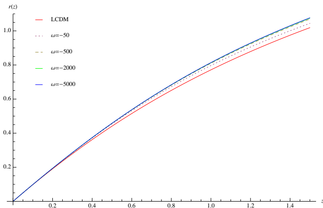
FIG. 2: The comoving distance r(z) as a function of redshift for different values of \omega .
