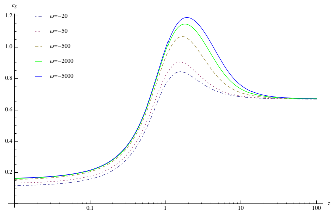
FIG. 3: Plot of c_s as a function of redshift for various values of the Brans-Dicke parameter. As can be seen during the transition to the accelerating phase the perturbations go superluminal for \omega \lesssim -190 .
