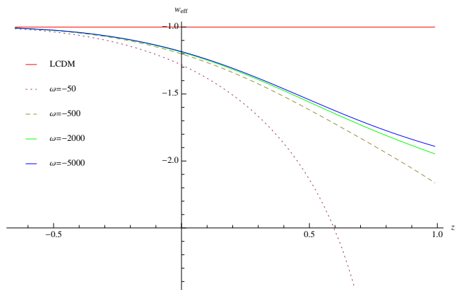
FIG. 1: The effective equation of state w_{\text{eff}} as a function of redshift for various values of the Brans-Dicke parameter.
