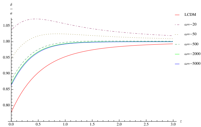
FIG. 4: The growth rate \frac{\delta}{a} as a function of redshift for different values of the BD parameter, \omega .
