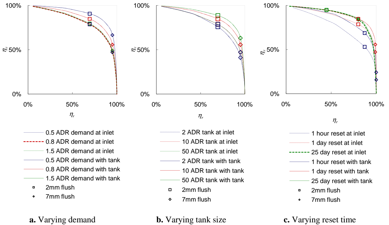
Figure 2: Removal vs volumetric efficiency graphs
