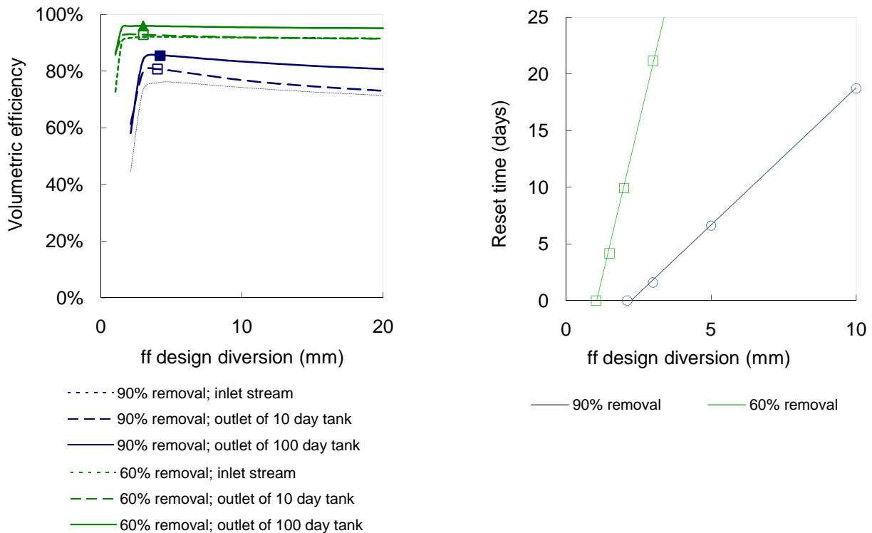
Figure 3: Optimal design diversions and reset times
