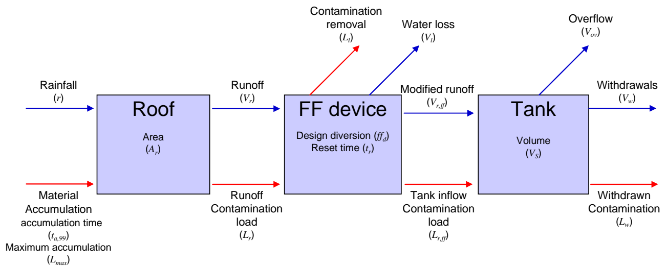
Figure 1: Contaminant and water flow through a RWH system with first-flush
