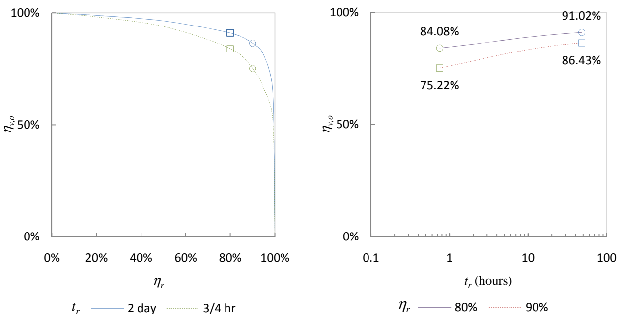
Figure 4: Difference in performance between a slow and fast resetting optimised first-flush device
