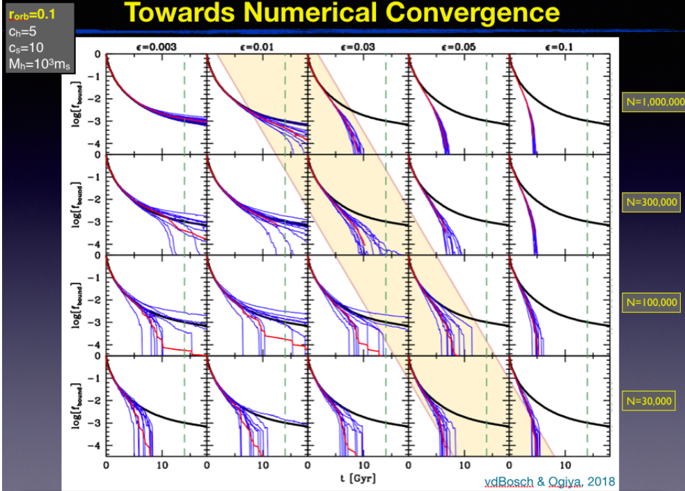
Figure 1: Bound fraction of mass as function of time for simulations with different mass resolution N_p and different force softening \epsilon . The black line shows the ‘converged’ results of a simulation with N_p = 10^7 and \epsilon = 0.003 ; the blue line the results from 10 simulations; the red line their average. @copyright: F. van den Bosch, private correspondence. For a detailed discussion of this figure, See van den Bosch and Ogiya (2018) , figure 10, 4077.
