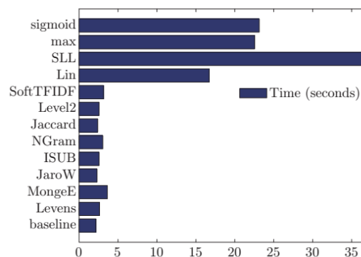
Fig. 4. Computation time on benchmarks data set
