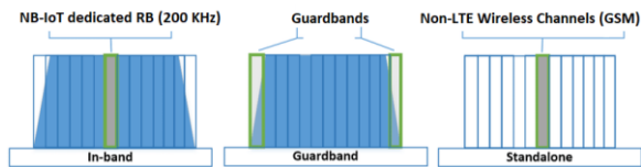
Fig. 2: NB-IoT operation mode
