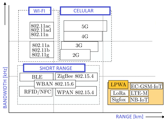
Fig. 1: Deployment with LPWA technology depending on range and width band
