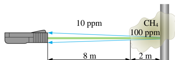
Fig. 1. Remote gas sensors based on the Tunable Diode Laser Absorption Spectroscopy (TDLAS) provide an integral measurement. Here the measurement would read 8 \text{ m} \cdot 10 \text{ ppm} + 2 \text{ m} \cdot 100 \text{ ppm} = 280 \text{ ppm} \cdot \text{m} .
