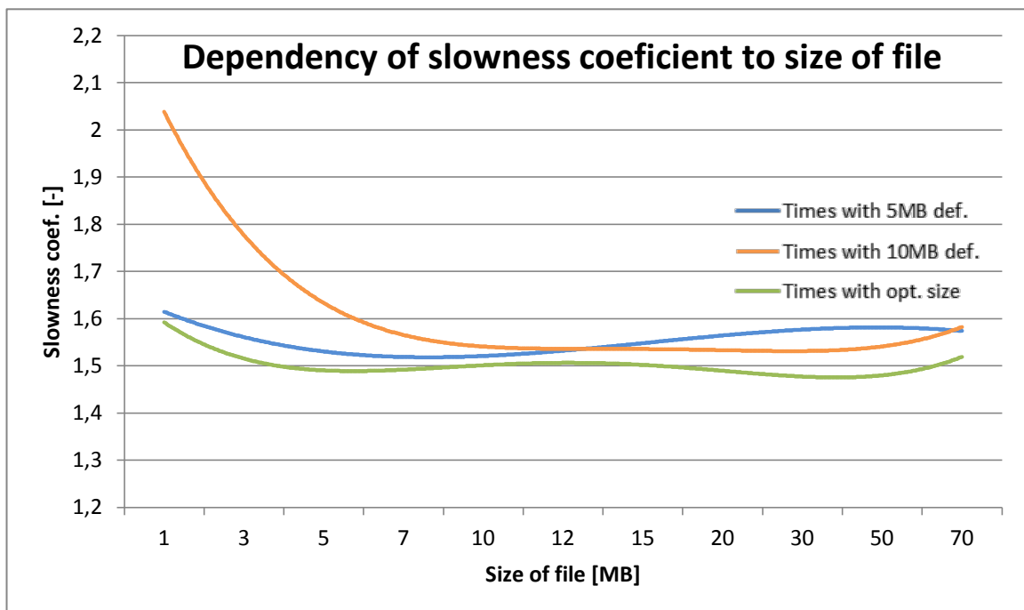
Graph 1: Dependency of slowness coefficient to size of file
