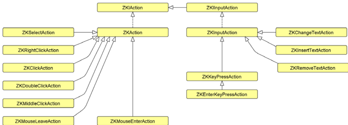
Figure 5: Actions diagram
