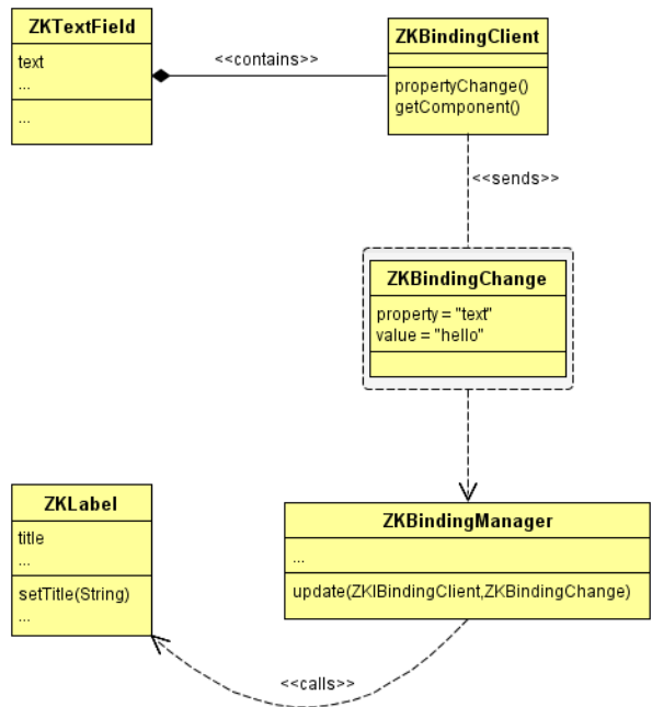
Figure 12: The binding diagram
