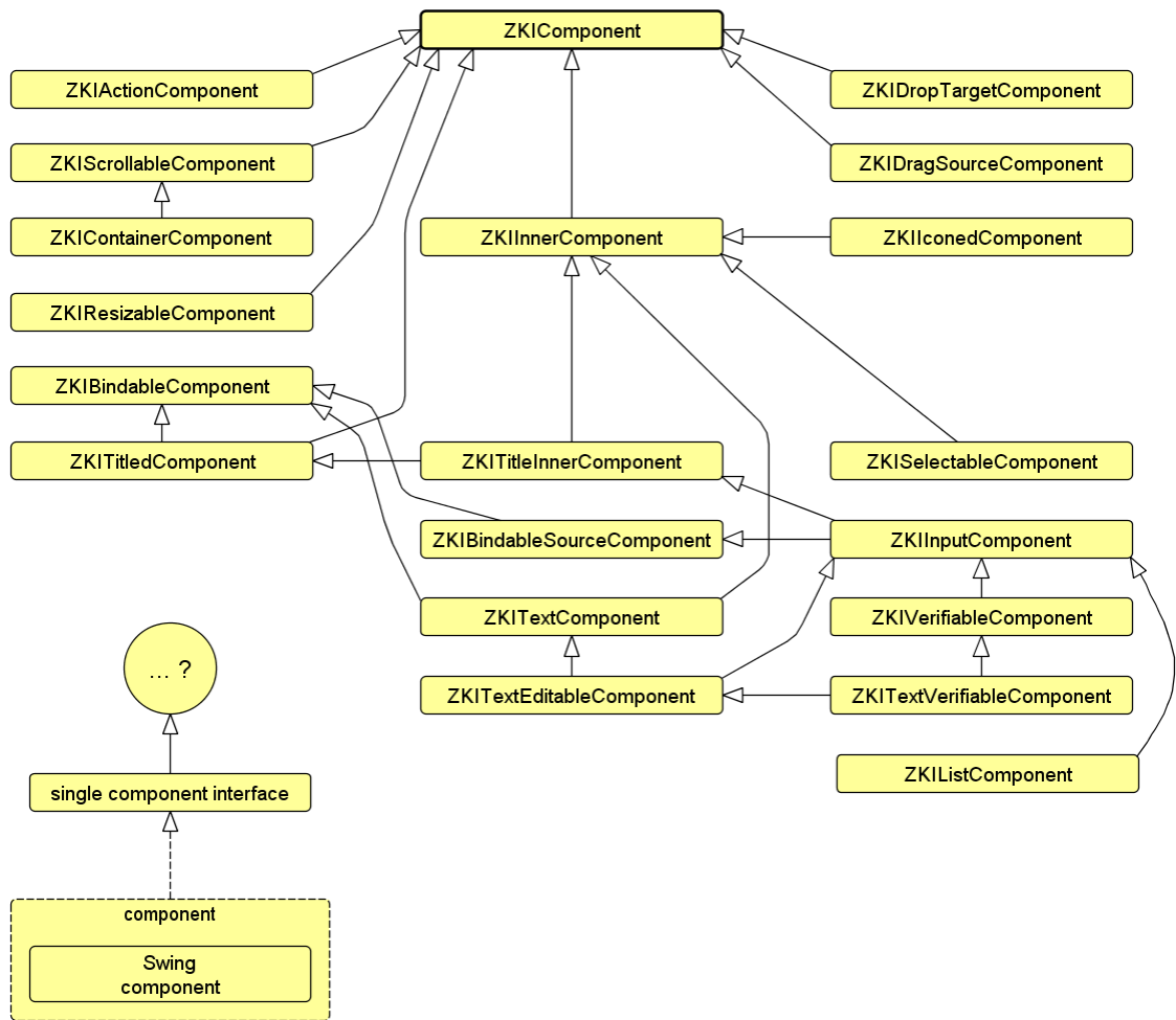
Figure 4: Tree of interfaces
