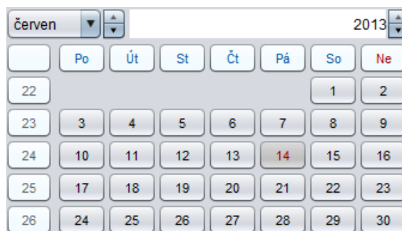
Figure 10: ZKCalendar component
