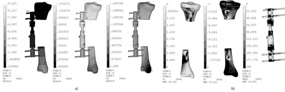
Fig. 16. Variant II: a) The displacements, b) The first and third principal stress – load state 3
