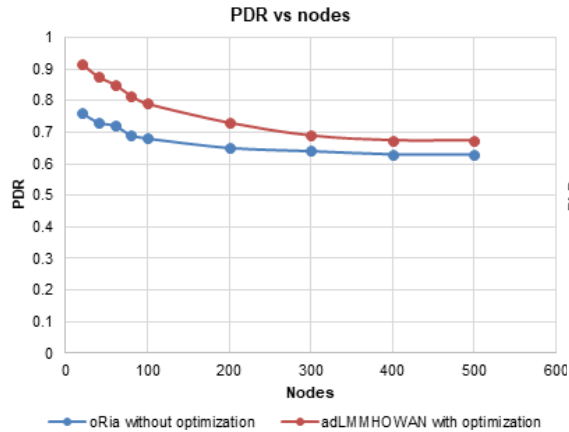
Figure 4. PDR performance for oRia and adLMMHOWAN multi-parameter AODVUU routing before and after Taguchi optimization mechanism
