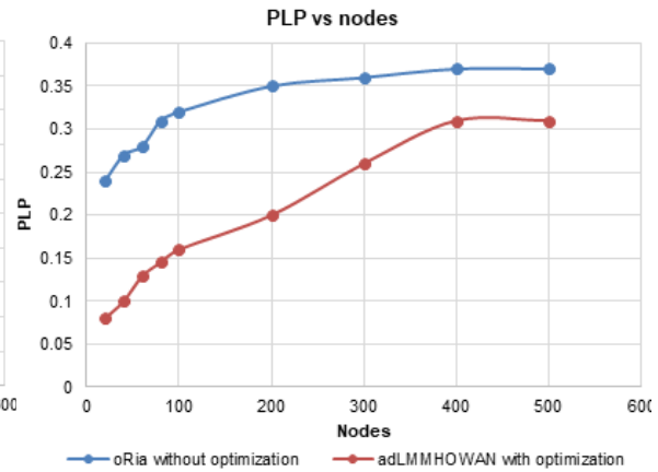
Figure 5. PLP performance for oRia and adLMMHOWAN multi-parameter AODVUU routing before and after Taguchi optimization mechanism
