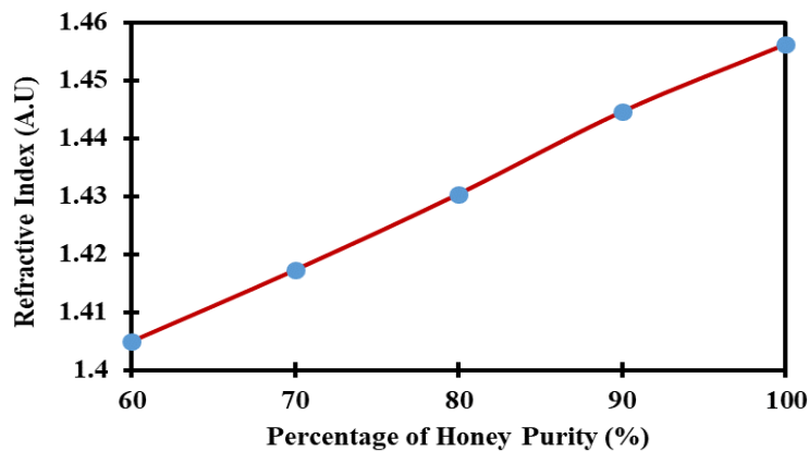
Figure 2. Refractive index of adulterated honey samples
