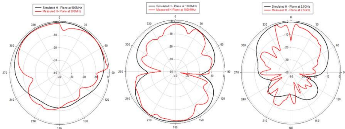
Figure 3b. Simulated vs Measured H- Plane Results in the UP mode at 900MHz, 1800MHz and 2.5GHz
