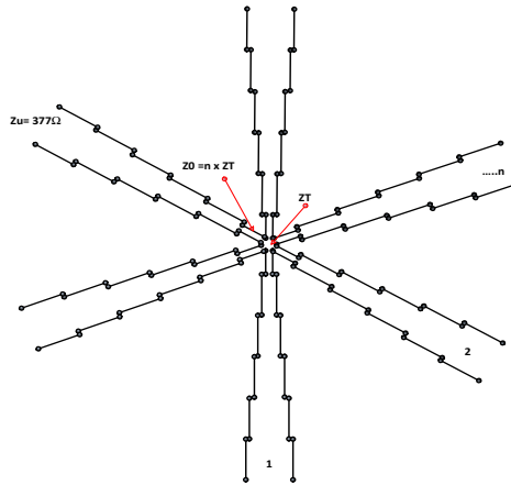
Figure 2. Antenna structure
