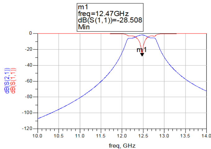
Figure 2. The response of filter dimensions in ADS
