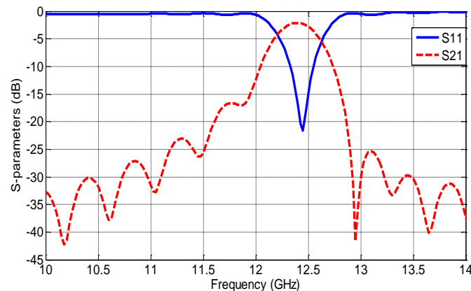
Figure 5. Simulated S-parameters of the filter using R03003 substrate
